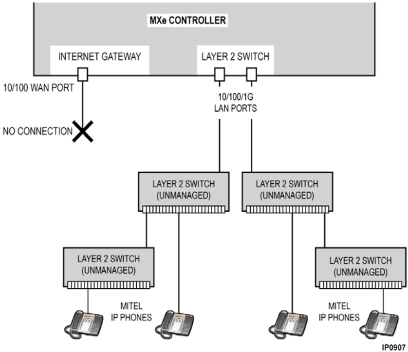
Figure 130: MXe Voice-Only Configuration Example
