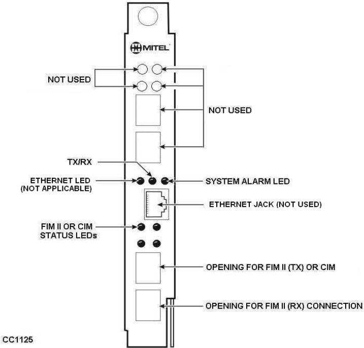
Figure 167: Peripheral Cabinet FIM LEDs
