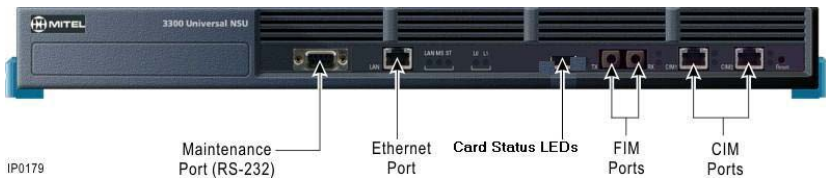
Figure 115: Universal NSU – Front Panel
