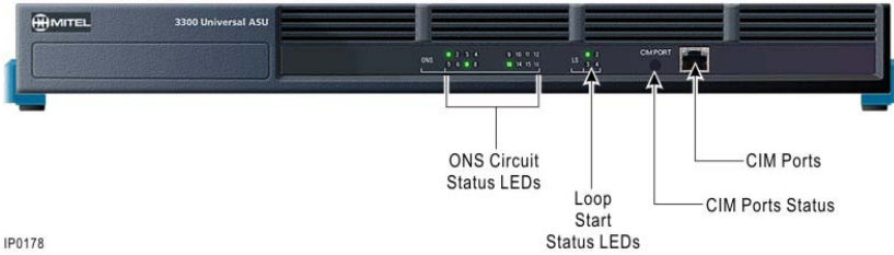
Figure 163: Universal ASU LEDs
