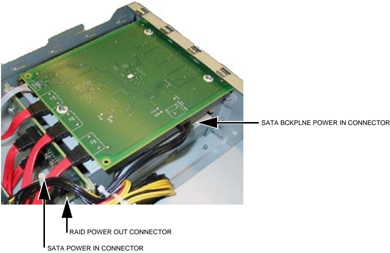
Figure 90: Power Connectors
