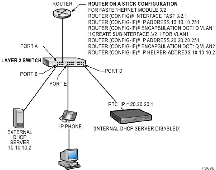
Figure 128: Configuration 3 Example
