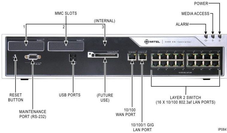
Figure 105: CXi Controller – Front Panel
