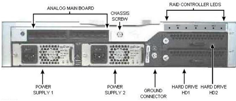
Figure 99: MXe Controller – Back Panel, Redundant
