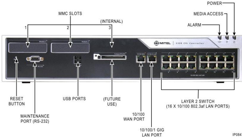
Figure 148: Controller LEDs (CX/CXi)
