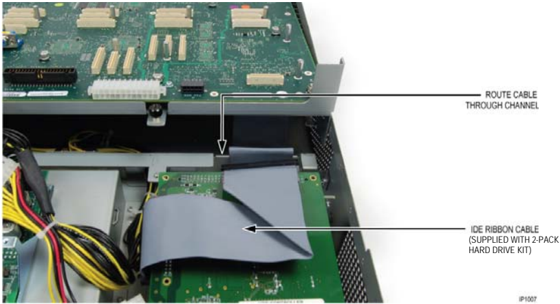
Figure 86: Routing the Pre-formed IDE Interconnect Cable
