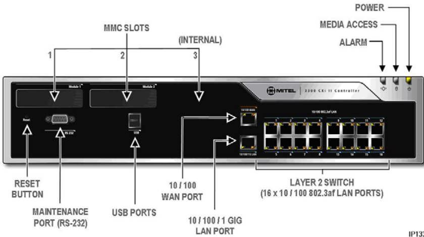
Figure 108: CXi II Controller - Front Panel
