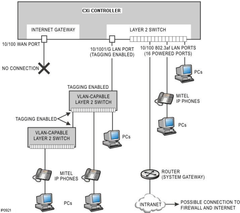
Figure 131: CXi/CXi II Voice and Data Configuration Example
