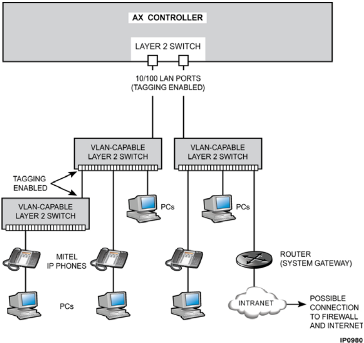
Figure 134: AX Voice and Data Configuration Example
