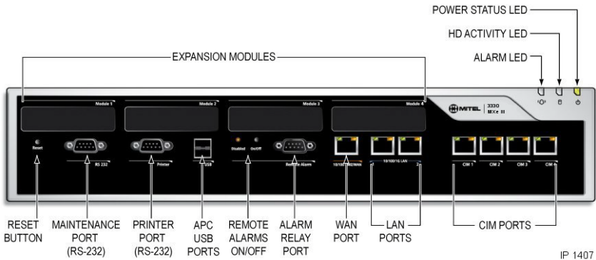
Figure 102: MXe Server – Front panel – CIM ports not used
