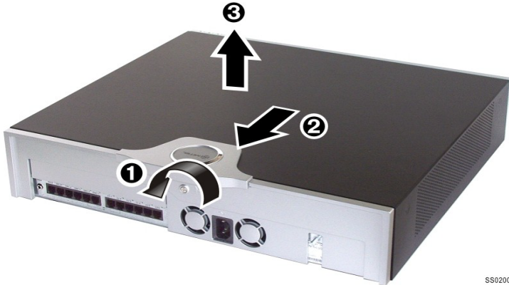
Figure 14: CX/CXi, CX II/CXi II - Removing the cover
