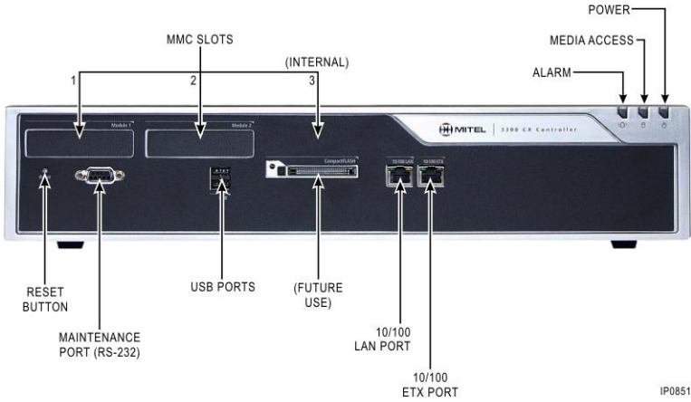
Figure 104: CX Controller – Front Panel
