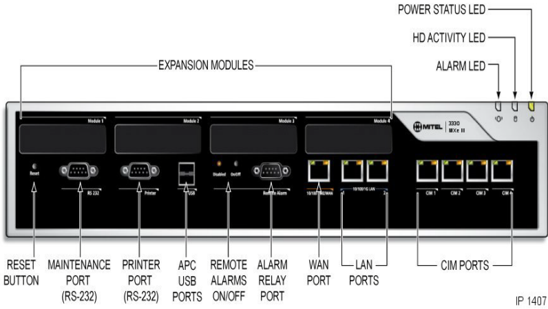
Figure 98: MXe Controller – Front Panel
