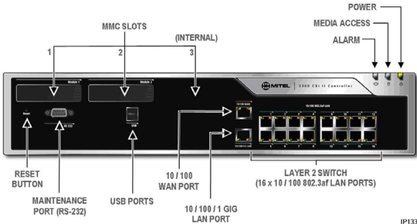
Figure 149: Controller LEDs (CX II/CXi II)
