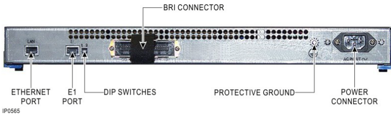
Figure 119: BRI NSU – Back Panel
