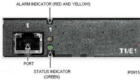
Figure 158: Controller T1/E1 Combo Card (Rel 6.0)
