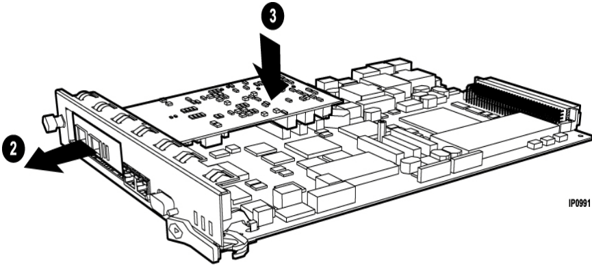
Figure 17: Slide in and seat module (AX)
