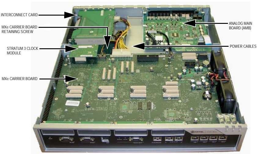
Figure 30: MXe II Controller with Top Cover Removed
