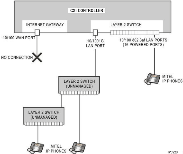
Figure 136: CXi/CXi II-based Typical Voice-Only Network
