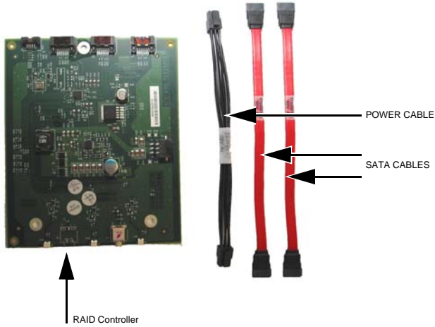
Figure 33: MXe III SATA RAID Controller and SATA Cables
