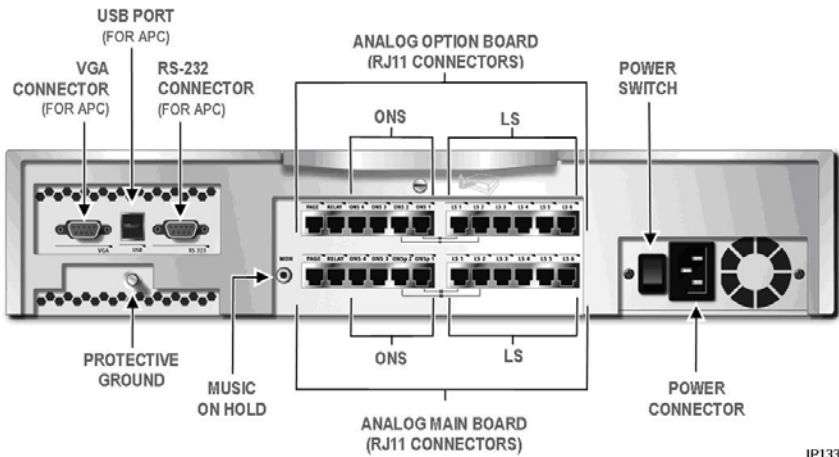
Figure 109: CX II and CX II - Back Panel
