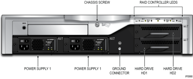
Figure 103: MXe Server – Back panel
