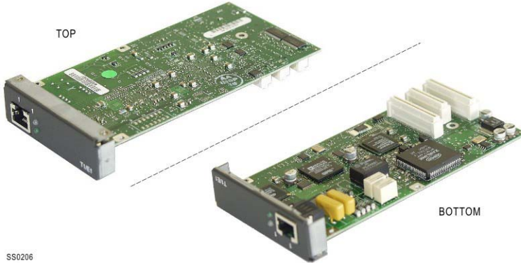
Figure 110: T1/E1 Combo Card (prior to Release 7.0)
