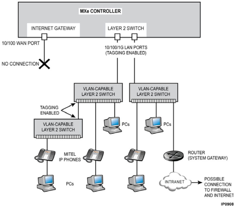
Figure 132: Mx e Voice and Data Configuration Example
