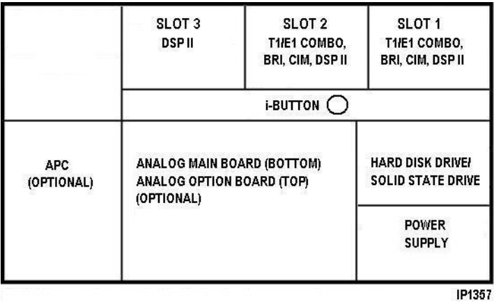
Figure 10: Slot Locations for the CX II Controller (without an Ethernet L2 Switch)
