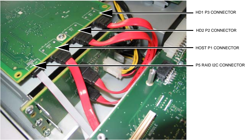
Figure 89: RAID Controller Connectors
