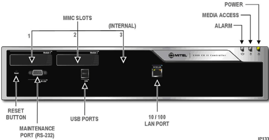
Figure 107: CX II Controller - Front Panel
