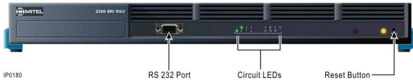
Figure 118: BRI NSU – Front Panel
