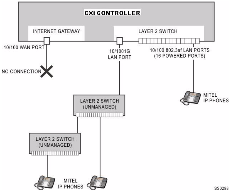
Figure 140: Expanded Voice only System
