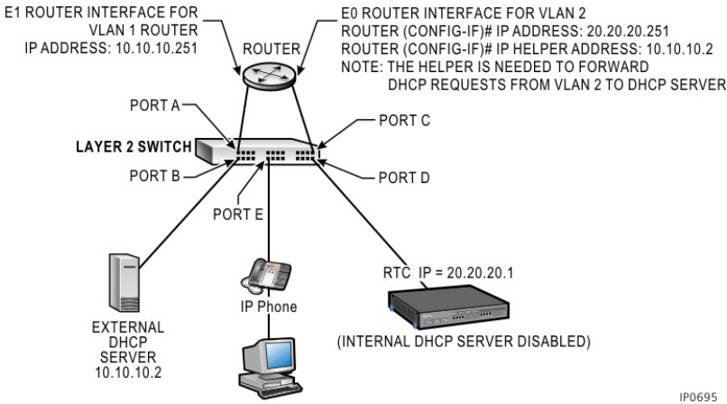
Figure 127: One DHCP Server for two VLANs - Example
