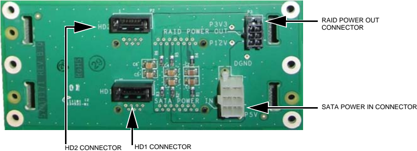
Figure 88: Hard Drive Backplane Connectors
