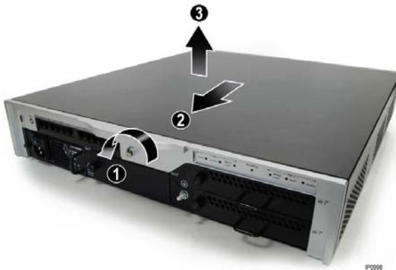
Figure 15: MXe/MXe Server - Removing the Cover
