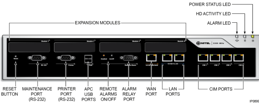
Figure 145: MXe/MXe Server – Front Panel
