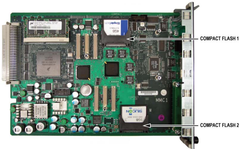
Figure 91: AX Flash 1 and Flash 2 Locations
