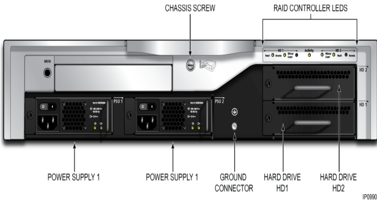
Figure 147: MXe Server – Rear Panel
