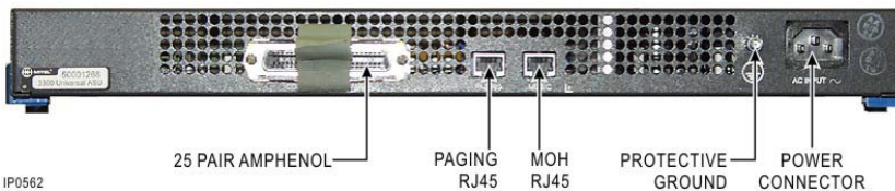
Figure 122: Universal ASU – Back Panel
