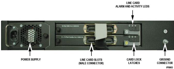
Figure 124: ASU II – Back Panel with a Line Card
