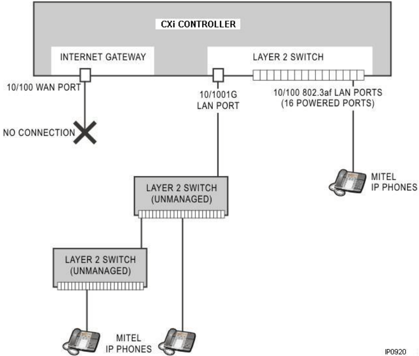
Figure 129: CXi/CXi II Voice-Only Configuration Example
