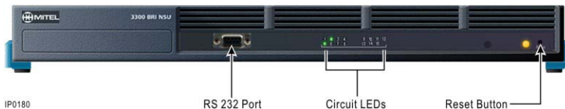
Figure 162: BRI NSU LEDs
