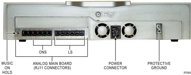
Figure 106: CX and CXi Controller – Back Panel
