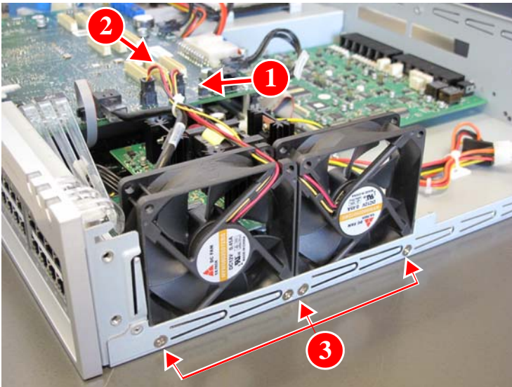
Figure 84: Fan Removal
