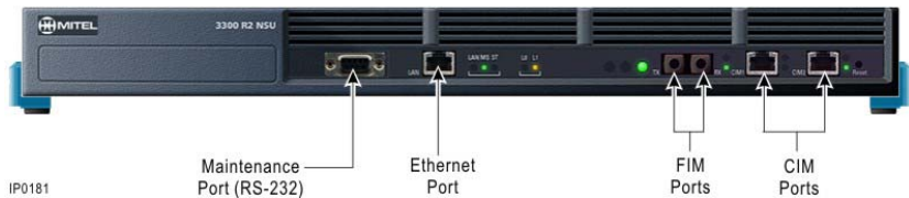
Figure 116: R2 NSU – Front Panel
