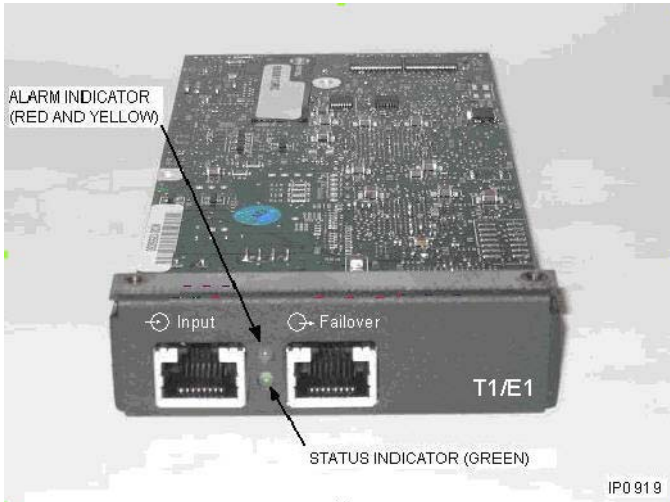
Figure 111: T1/E1 Combo Card - Resilient, from Release 7.0
