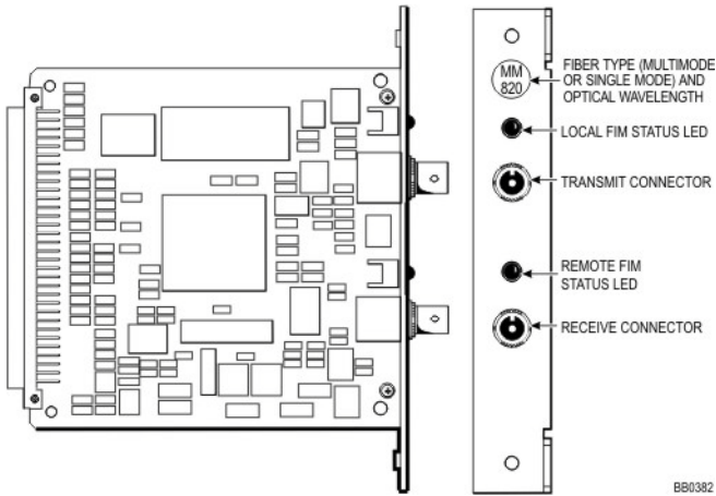
Figure 166: Peripheral Cabinet FIM LEDs
