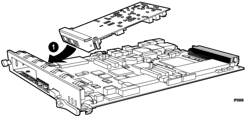
Figure 16: Position module at an angle (AX)
