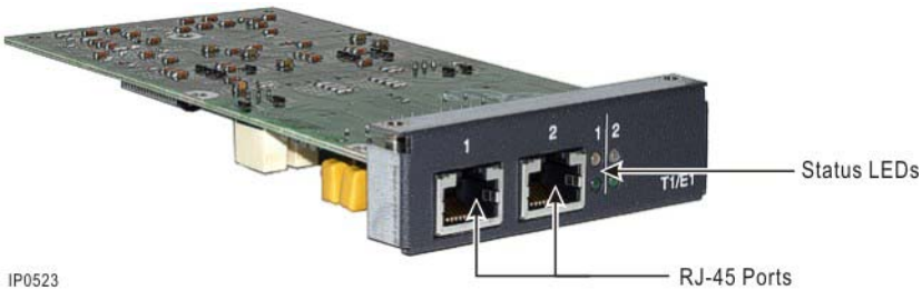
Figure 157: Dual T1/E1 Framer Module
