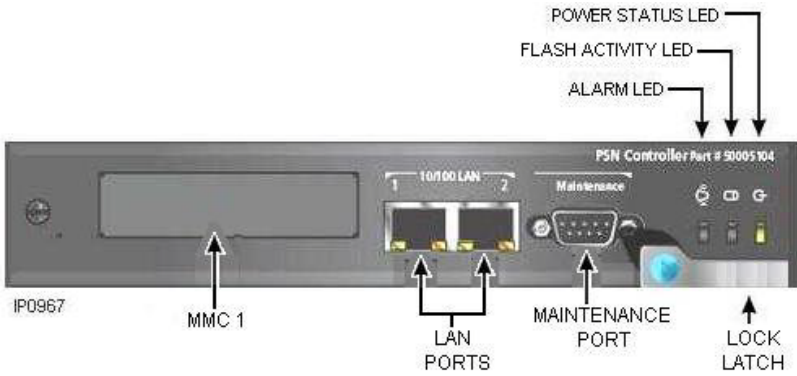
Figure 96: AX Controller Card View
