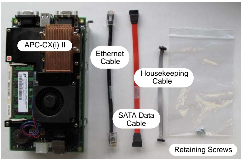
Figure 65: APC-CX(i) II Assembly Kit Components
