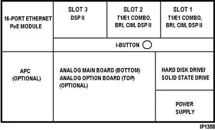
Figure 9: Slot Locations for the CXi II Controller (with an Ethernet L2 Switch with POE)
