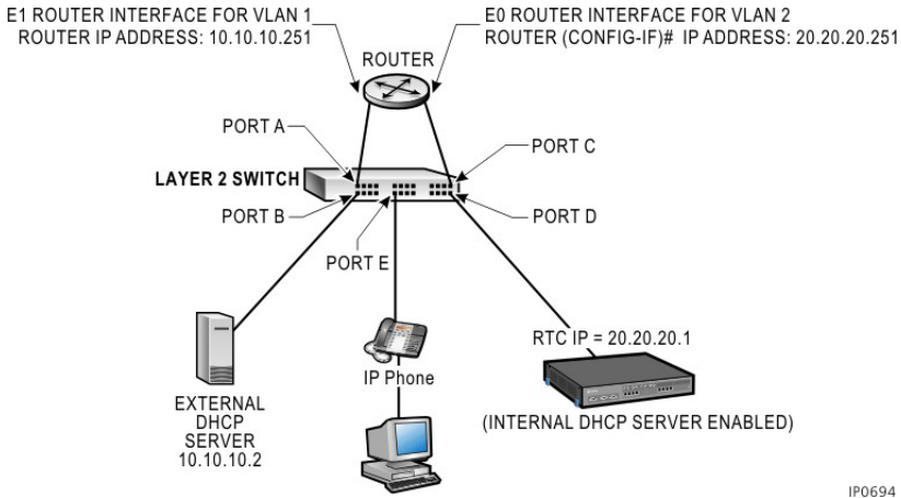
Figure 126: One DHCP Server per VLAN - Example
