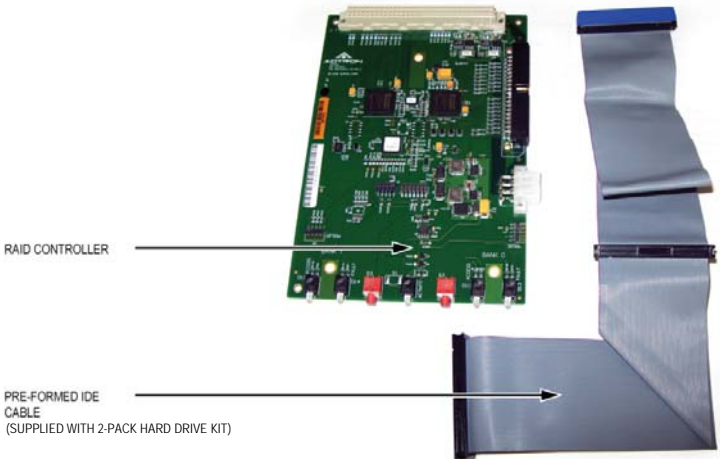
Figure 32: MXe II PATA RAID Controller and Pre-formed IDE Cable
