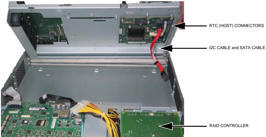
Figure 75: Disconnecting the I2C Ribbon Cable and the SATA Cable - MXe III
