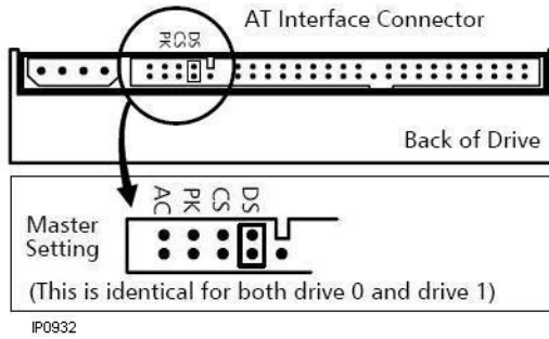
Figure 101: MXe II Controller – Hard Drive Jumper Settings
