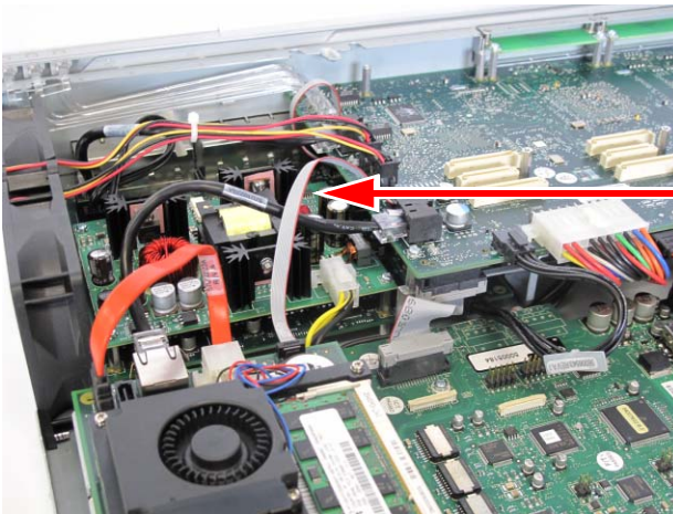
Figure 70: Cable Routing
