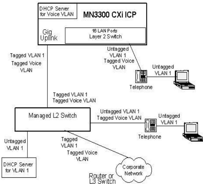
Figure 135: CXi/CXi II VLAN Behavior
