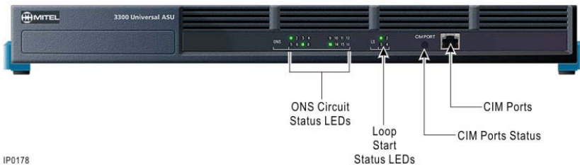
Figure 121: Universal ASU – Front Panel
