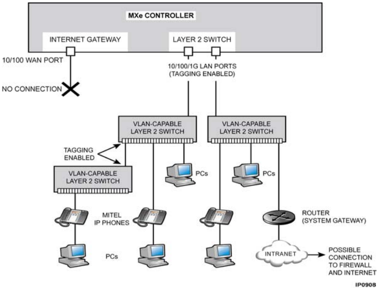
Figure 139: MXe-based Typical Voice and Data Network
