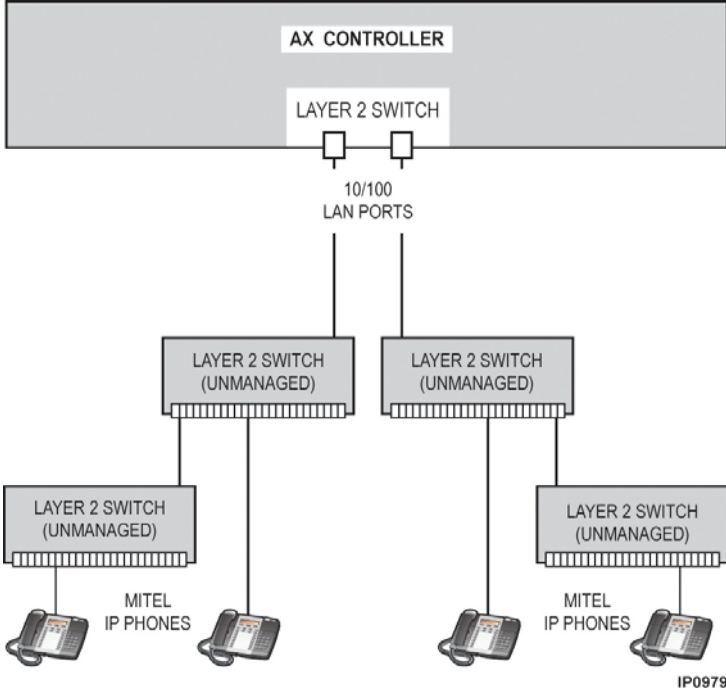
Figure 133: AX Voice-Only Configuration Example
