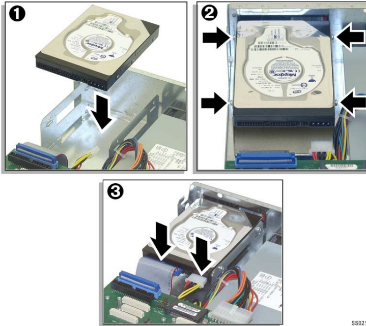
Figure 77: CX Controller Hard Drive Installation
