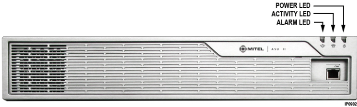
Figure 123: ASU II – Front Panel
