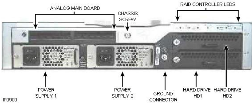
Figure 146: MXe Controller – Rear Panel with Analog
