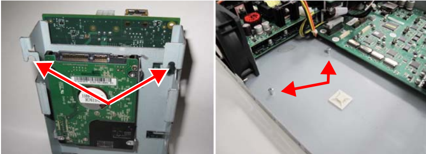
Figure 68: Notches and Shoulder Bolts
