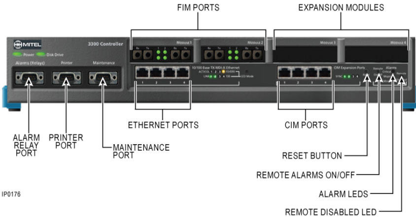
Figure 150: Controller LEDs (LX; MX; 100-User; 250/700-User)
