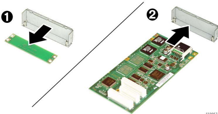
Figure 40: Attaching Cover Plate to the DSP Module
