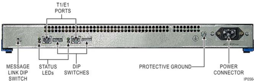
Figure 117: Universal/R2 NSU – Back Panel
