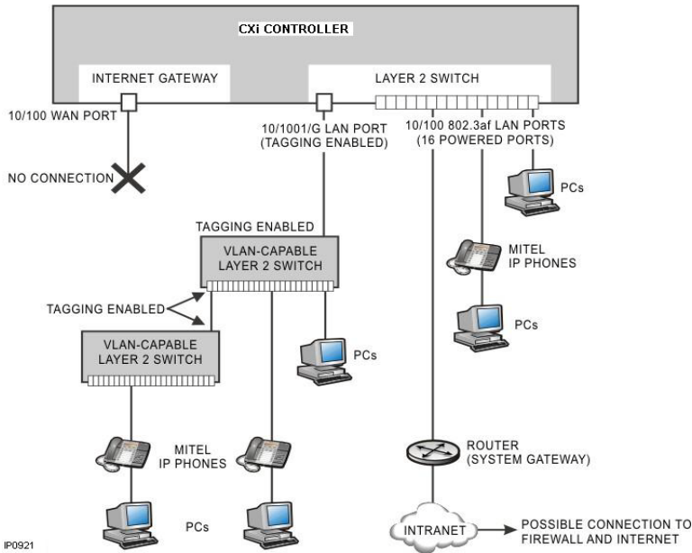
Figure 138: CXi/CXi II-based Typical Voice and Data Network
