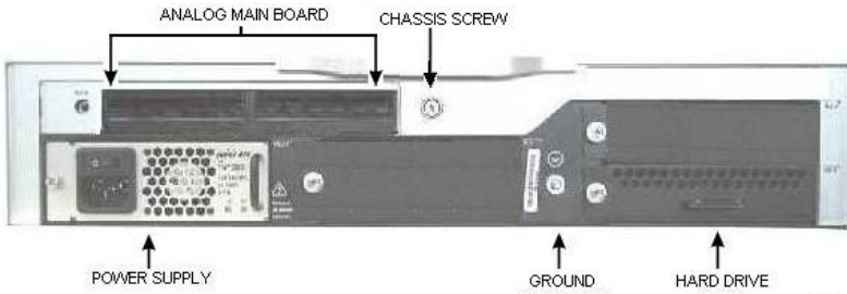
Figure 100: MXe Controller – Back Panel, Non-Redundant
