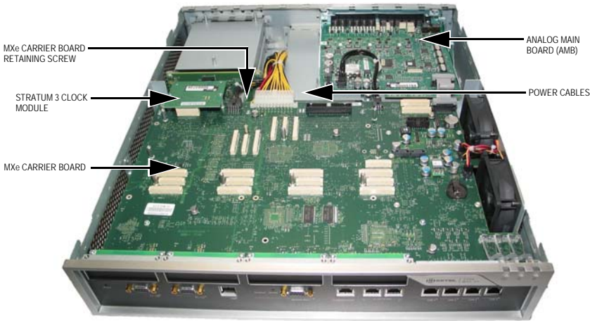
Figure 31: MXe III Controller with Top Cover Removed
