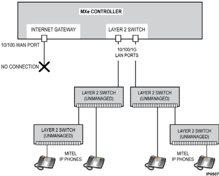
Figure 137: MXe-based Typical Voice-Only Network
