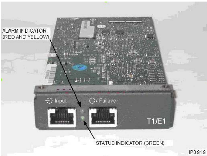
Figure 159: Resilient T1/E1 Combo Card (Rel 7.0)
