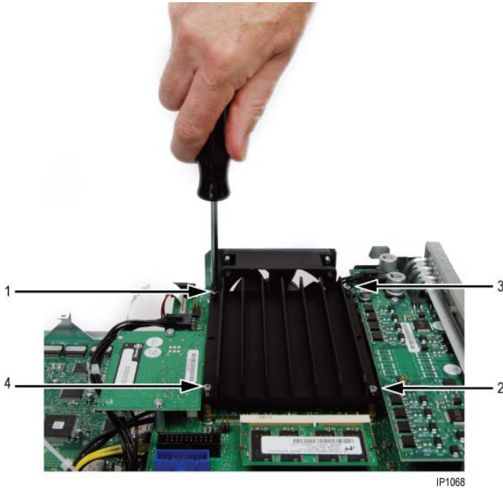
Figure 63: Tightening the Screws
