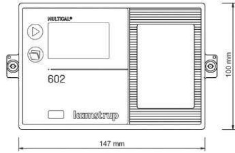
MULTICAL® 602's front dimensions
