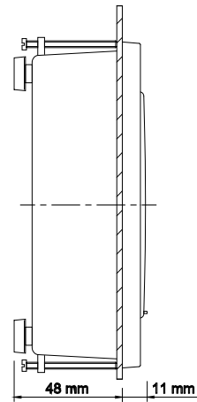
Panel-mounted MULTICAL® 602 seen from the side
