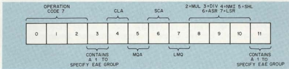
Figure 8 EAE Microinstruction Format
