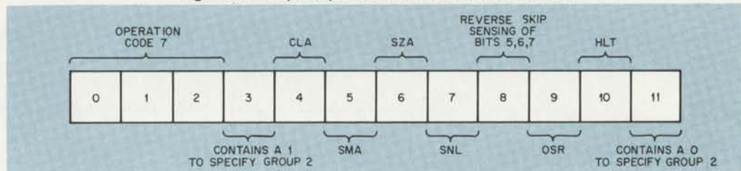
Figure 7 Group 2 Operate Microinstruction Format
