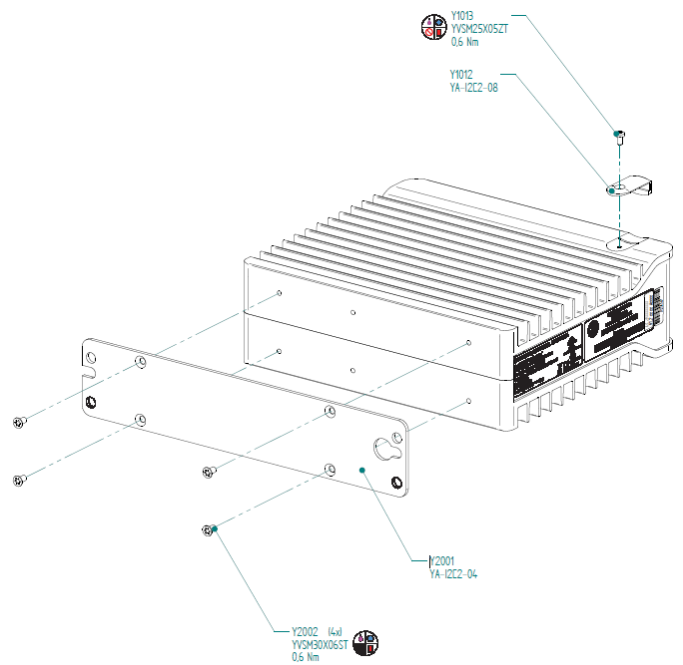
Figure 21: Panel-Mount Bracket Assembly CPE400
