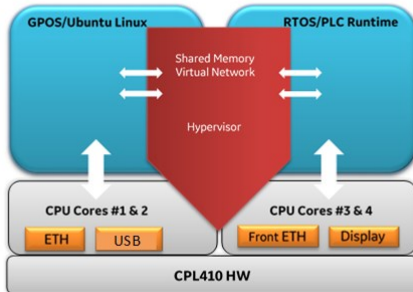
Figure 3: CPL410 Hardware/Software Separation
