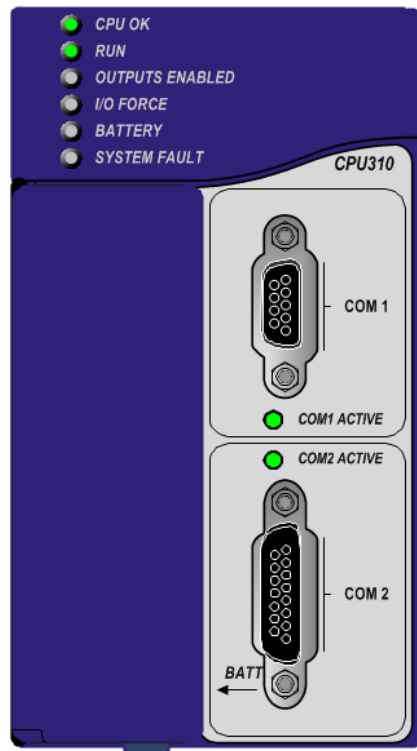
Figure 32: CPU310 Front View
