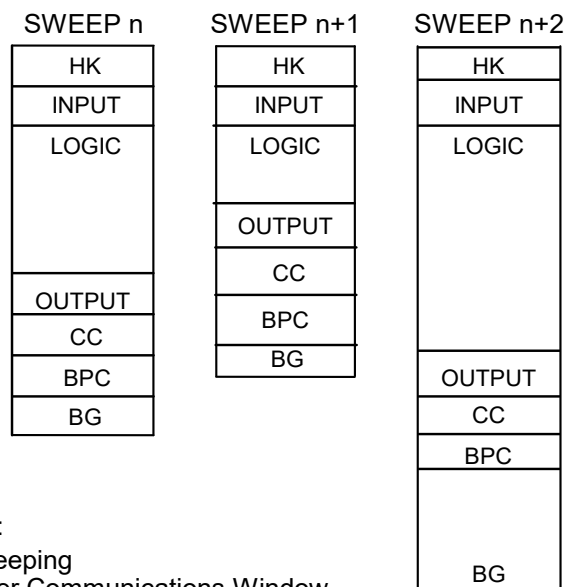
Figure 41: Typical Sweeps in Normal Sweep Mode
