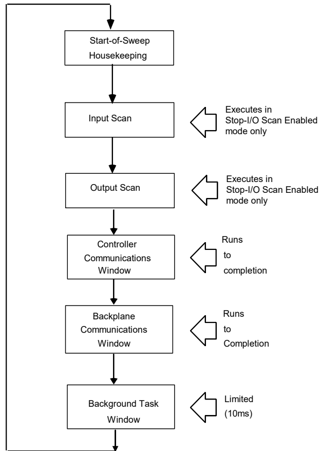
Figure 44: CPU Sweep in Stop-I/O Disabled and Stop-I/O Enabled Modes
