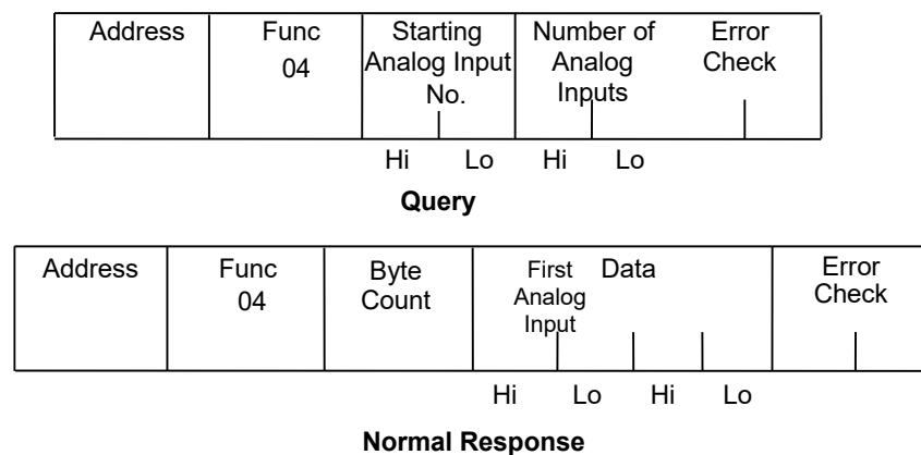
Figure 56: RTU Read Analog Inputs Message Format
