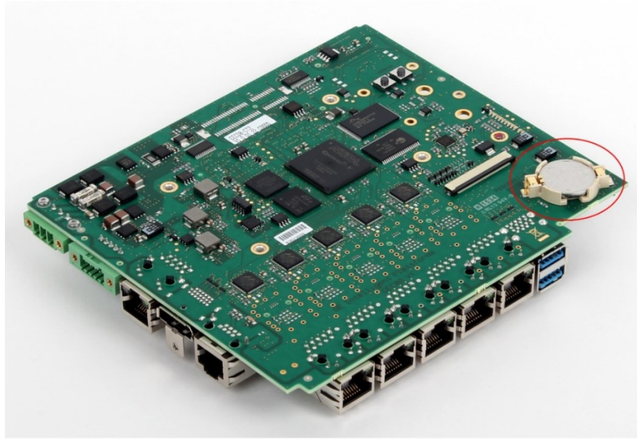
Figure 19: Location of RTC Battery on CPE400
