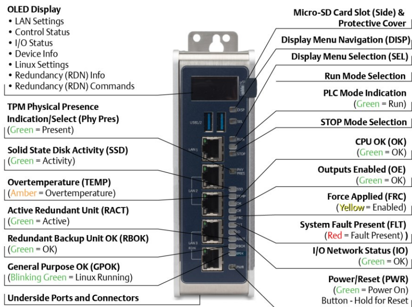
Figure 6: CPE400 Front View and Features
