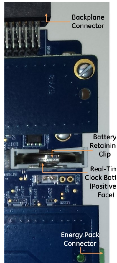
Figure 24: Location and Orientation of Real-Time Clock Battery in CPE330
