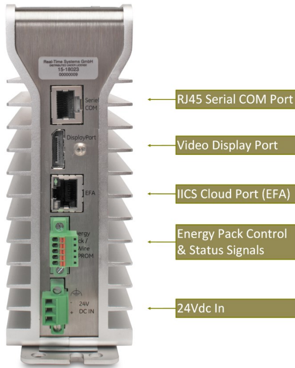
Figure 7: CPE400 Underside Ports & Connectors
