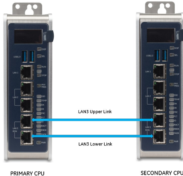
Figure 17: LAN3 Interconnects for Hot Standby Redundancy
