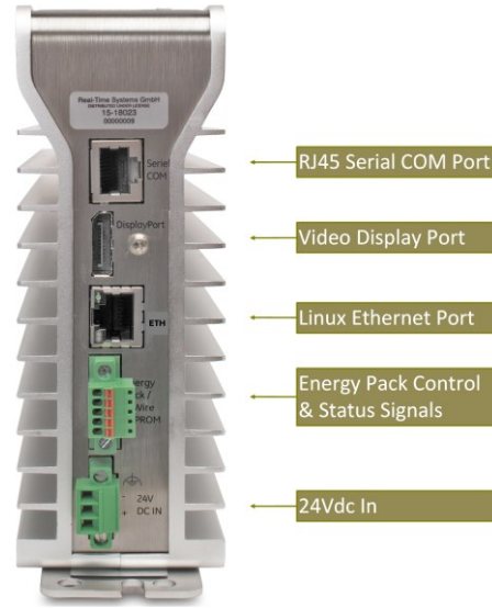
Figure 4: Underside Ports & Connectors
