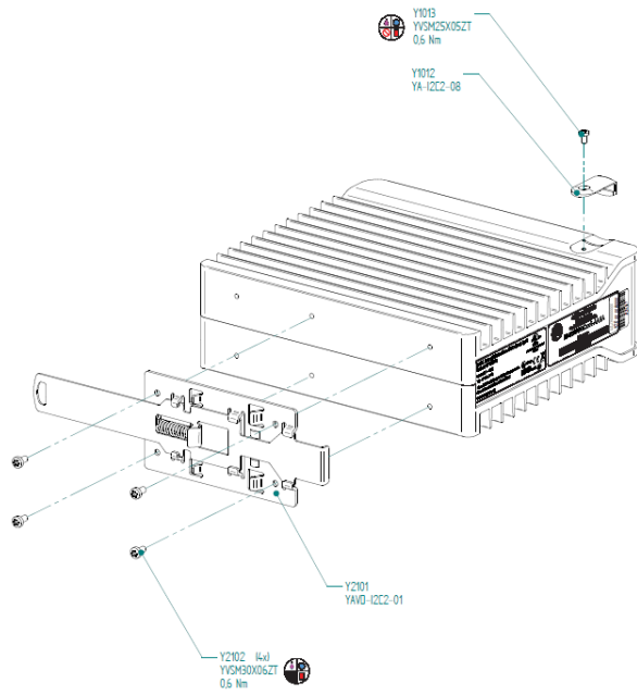
Figure 20: Din Rail Mount Bracket Assembly CPE400
