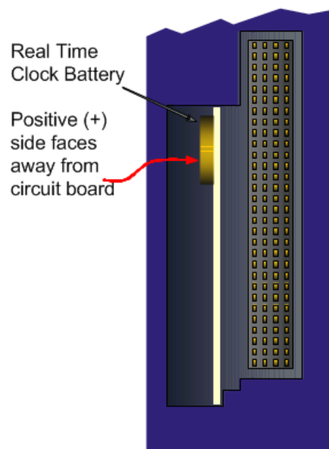
Figure 29: Accessing Real-Time Clock Battery (CPE302, CPE305, and CPE310)
