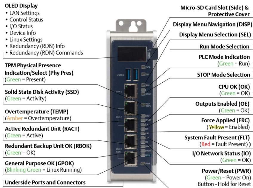
Figure 2: CPL410 Front View and Features
