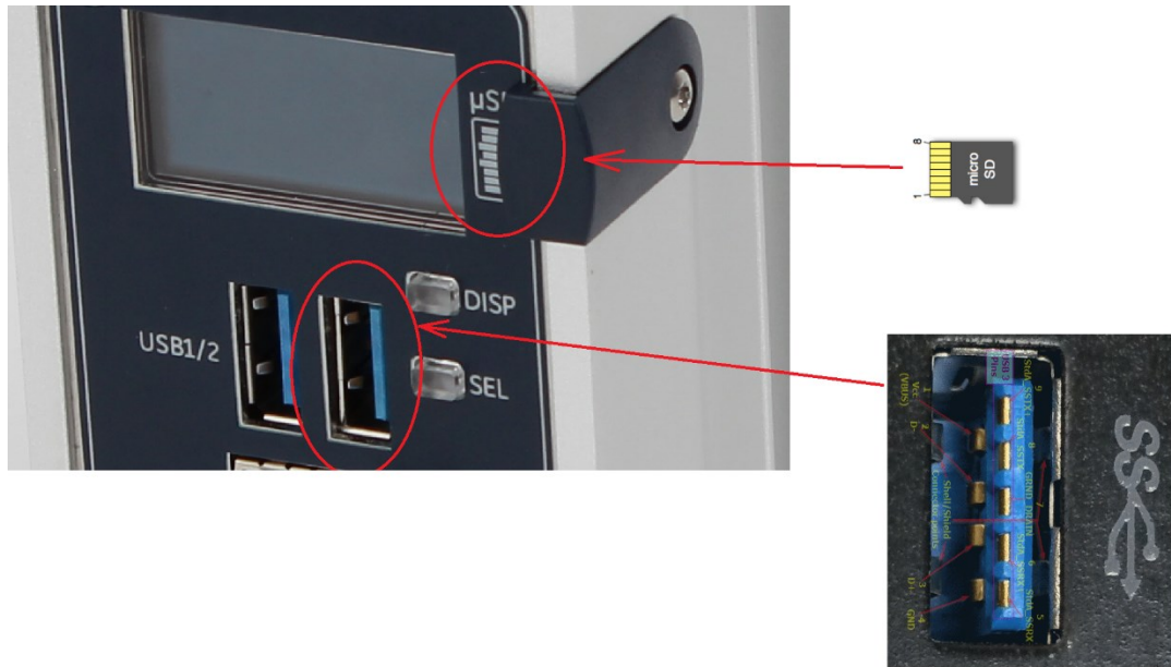
Figure 8: CPE400 Micro-SD & USB Pinouts
