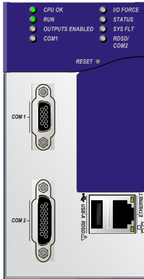
Figure 26: IC695CPE310 Front View
