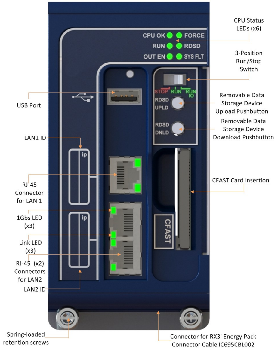
Figure 22: Front Display Port
