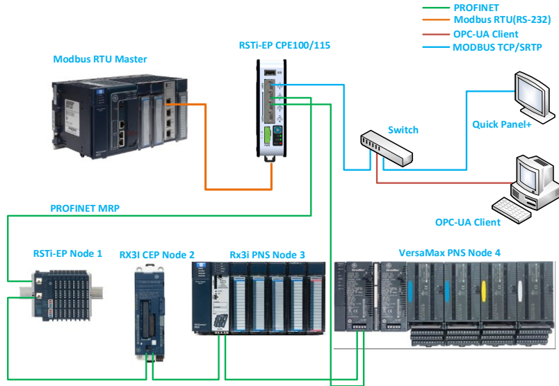
Figure 36: Typical Multi-Tier LAN Application (Star/Bus Topology)
