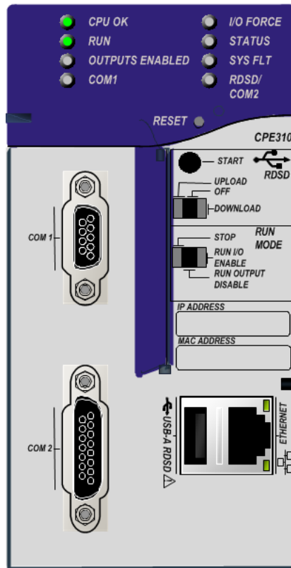
Figure 28: External Features of CPE310
