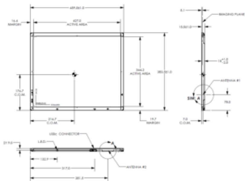
Figure 65 4336W-G5 X-ray Detector Dimensions in mm
