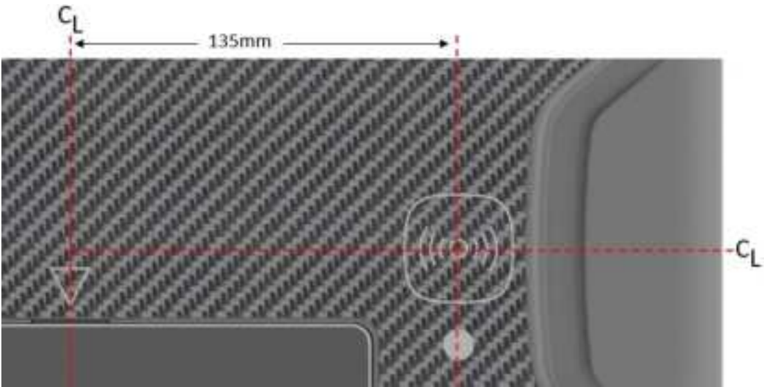
Figure 19 Third-party Inductive Battery Charger 4343W/4336W-G5/2530W-G5 X-ray Detector Alignment
