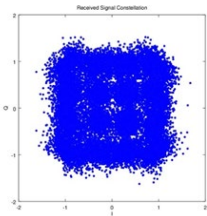
Figure 9: STC Correction Processing ( \tau = 0.2 T_d )
