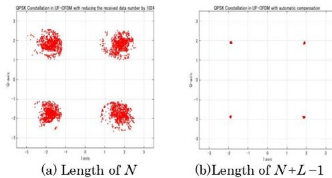
Figure 5 QPSK Demodulation Characteristics
