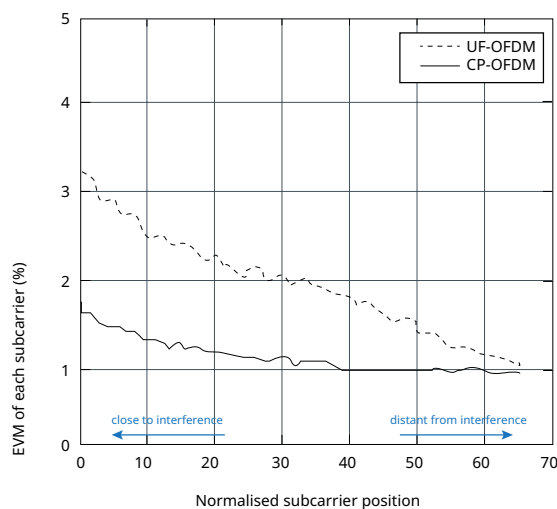
Figure 18: Interference evaluation by EVM
