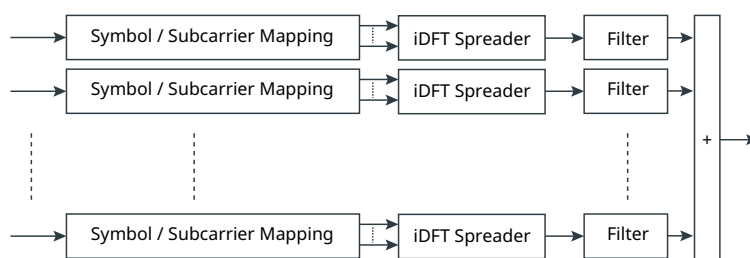
Figure 1: UF-OFDM Modulation Function Block Diagram
