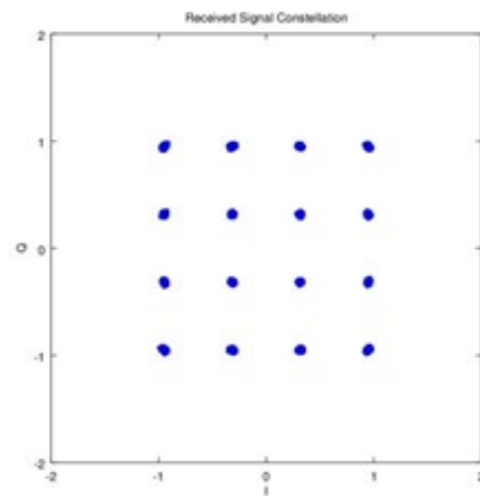
Figure 10: STC Correction Processing ( \tau = 0.01 T_d )
