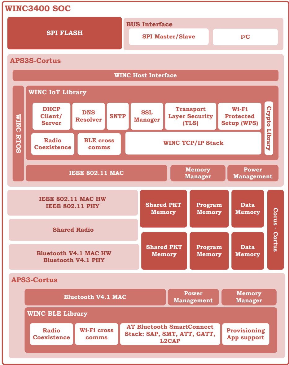
Figure 5-1. WINC System Architecture
