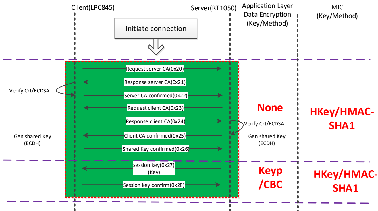
Figure 8. Asymmetric connection
