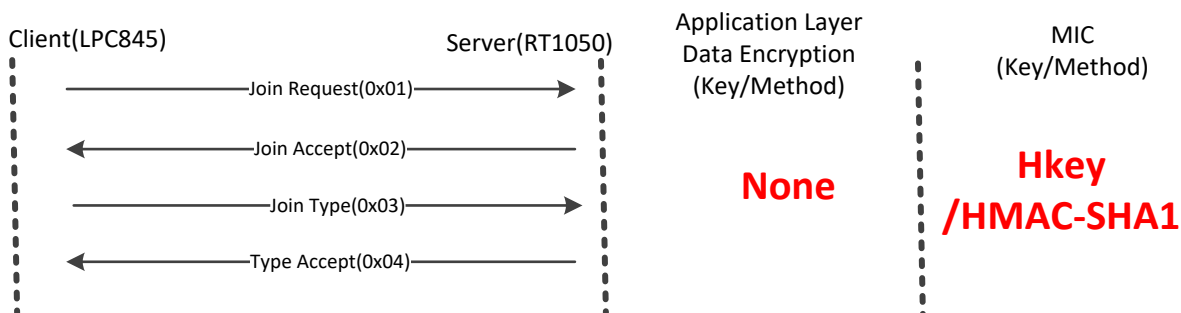
Figure 6. Initiate connection
