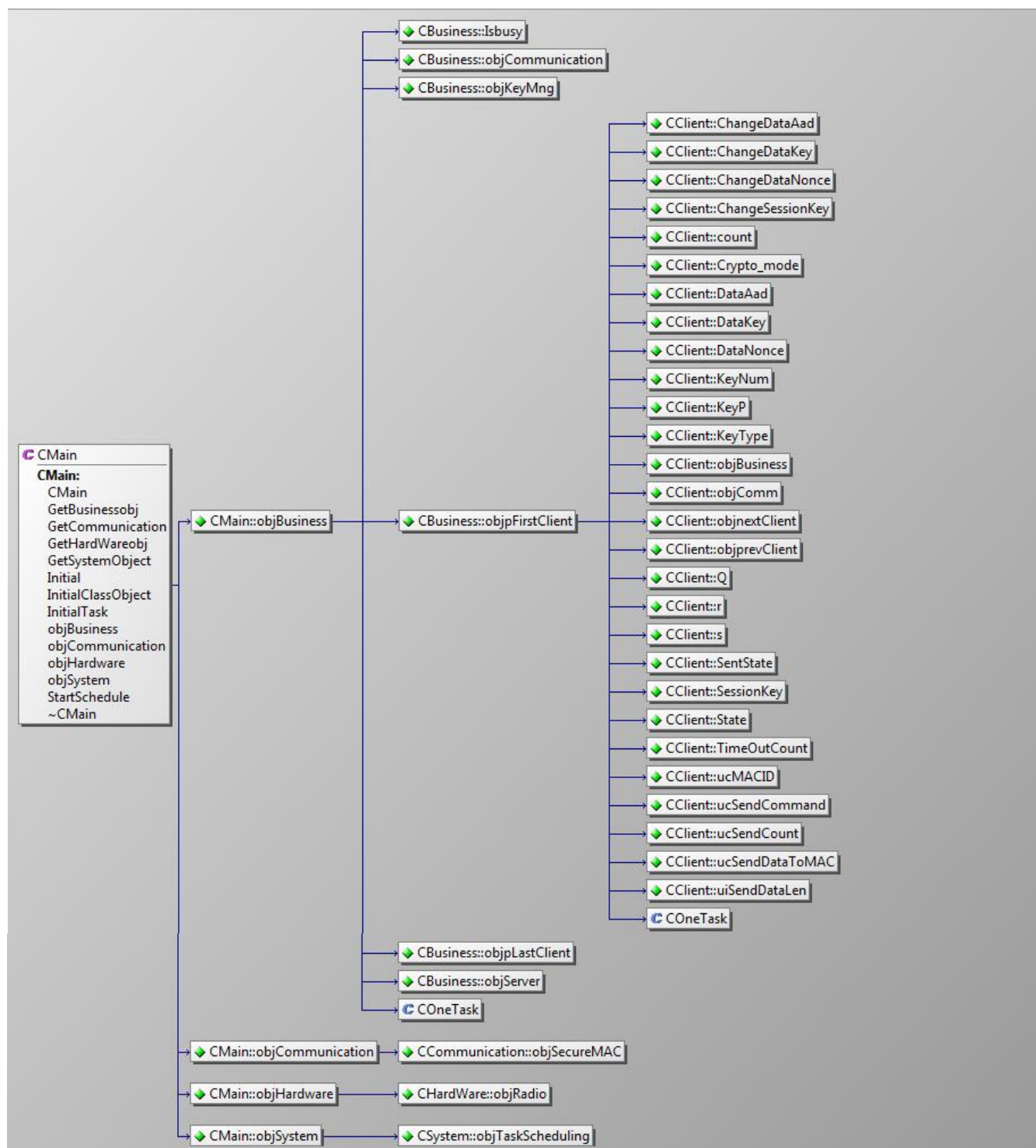
Figure 3. C++ Framework
