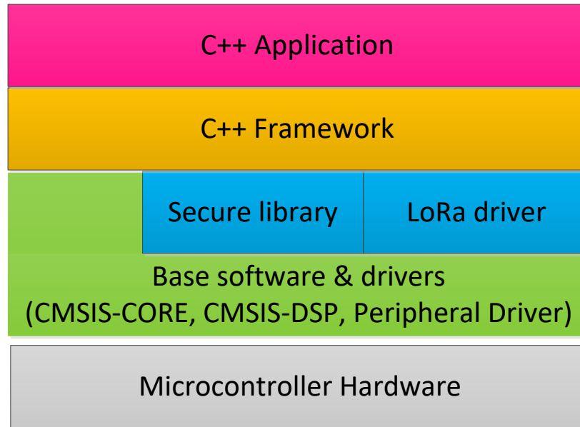
Figure 2. Software Architecture
