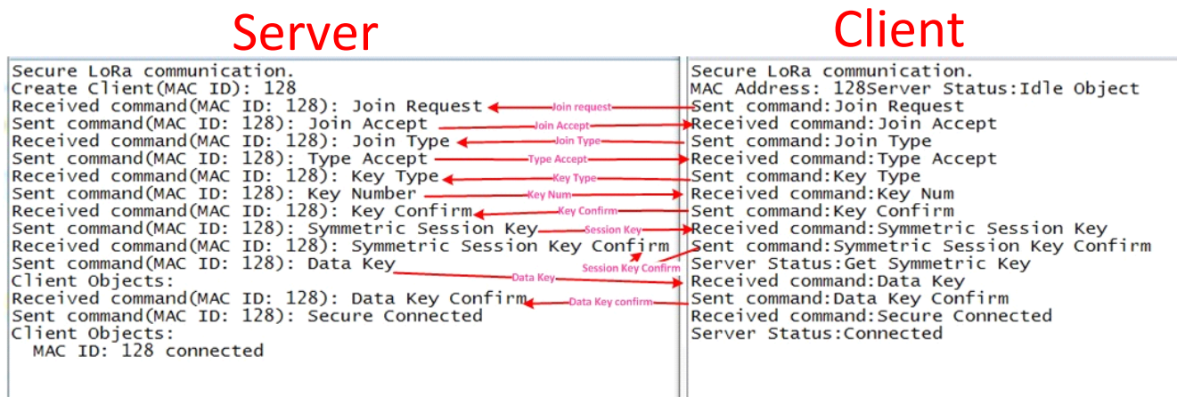
Figure 17. Symmetric connection
