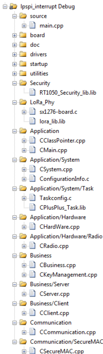
Figure 13. Server software
