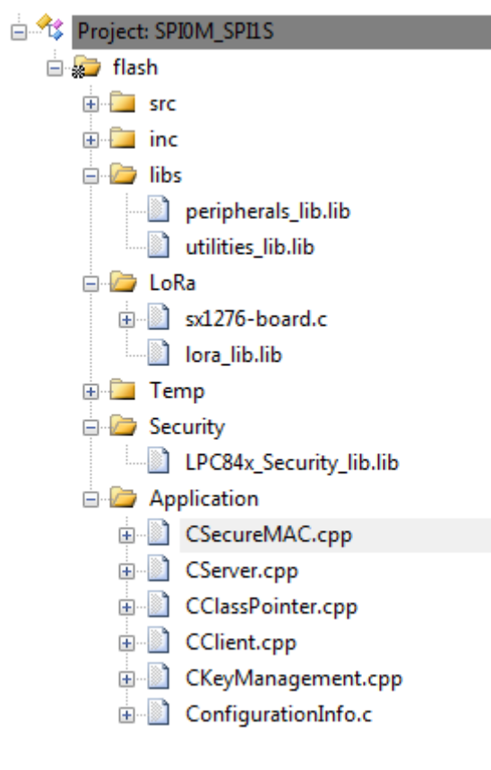
Figure 14. Client software
