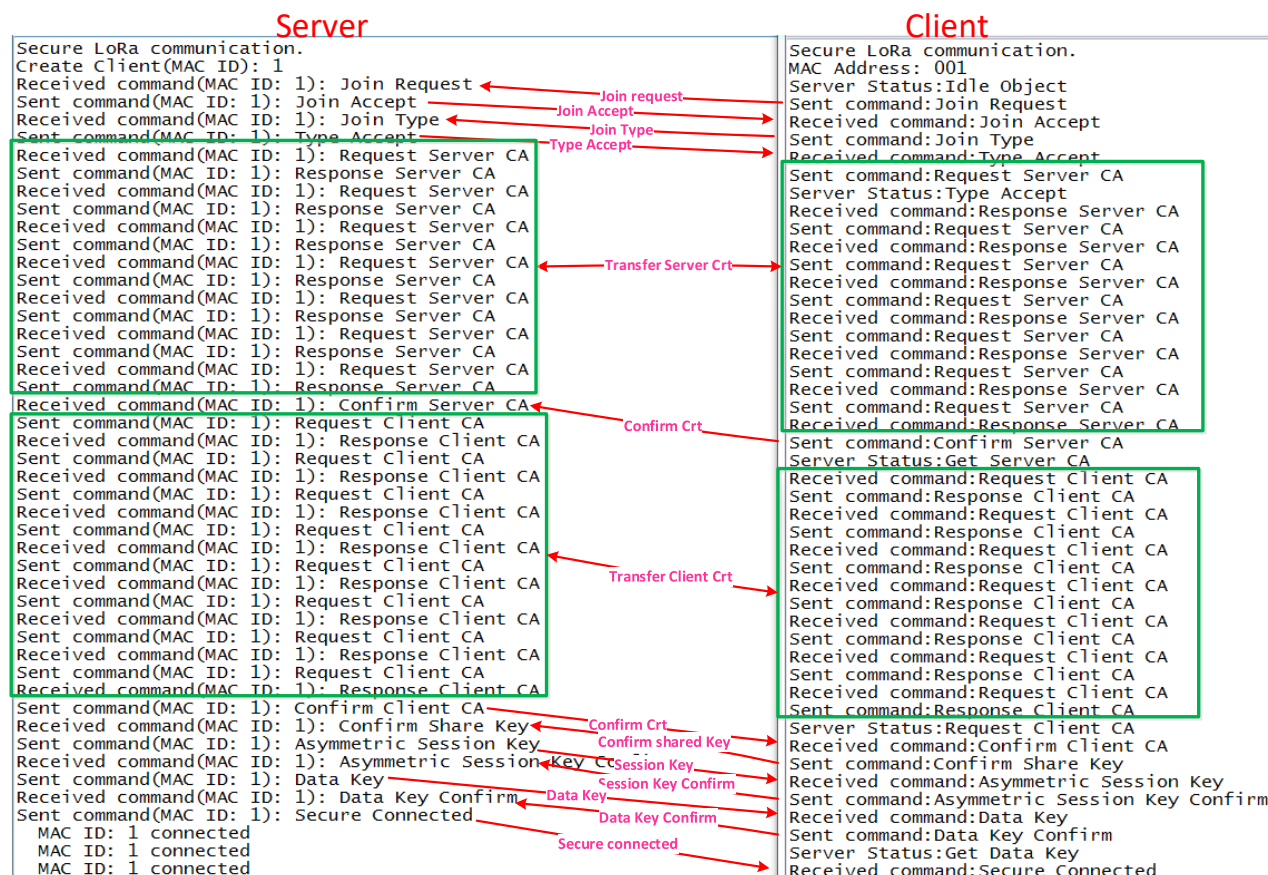
Figure 16. Asymmetric connection
