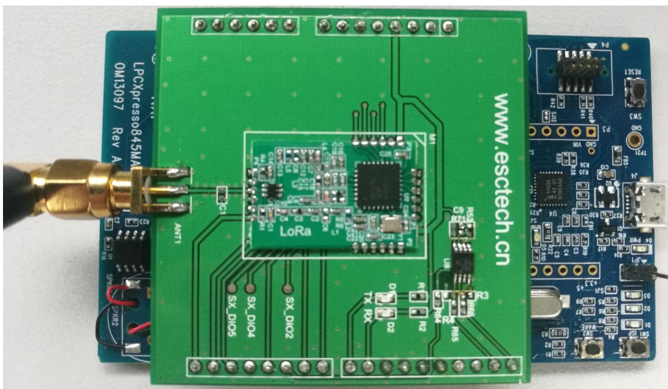
Figure 12. Client hardware
