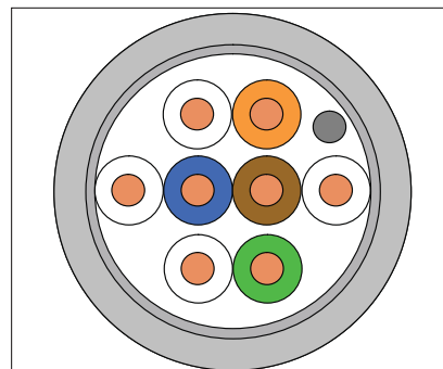
Category 5e PVC Shielded Cable
