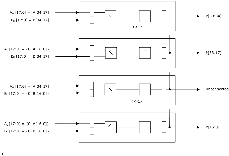
Figure 65 • Non-Pipelined Implementation Using Cascade Chain
