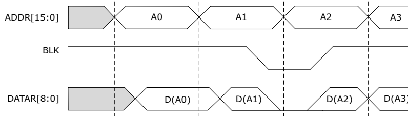
Figure 39 • Read Operation in \mu PROM
