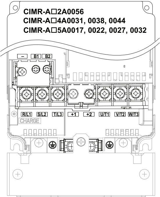
A1000 Main Circuit Terminal Configuration
