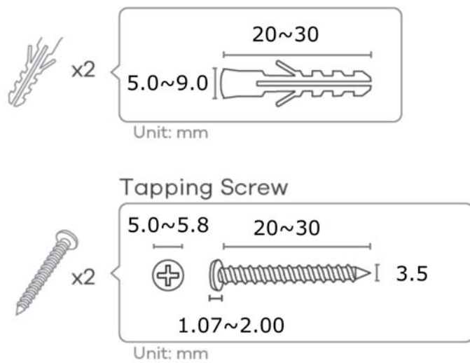
Figure 3 M3.5 Screw
