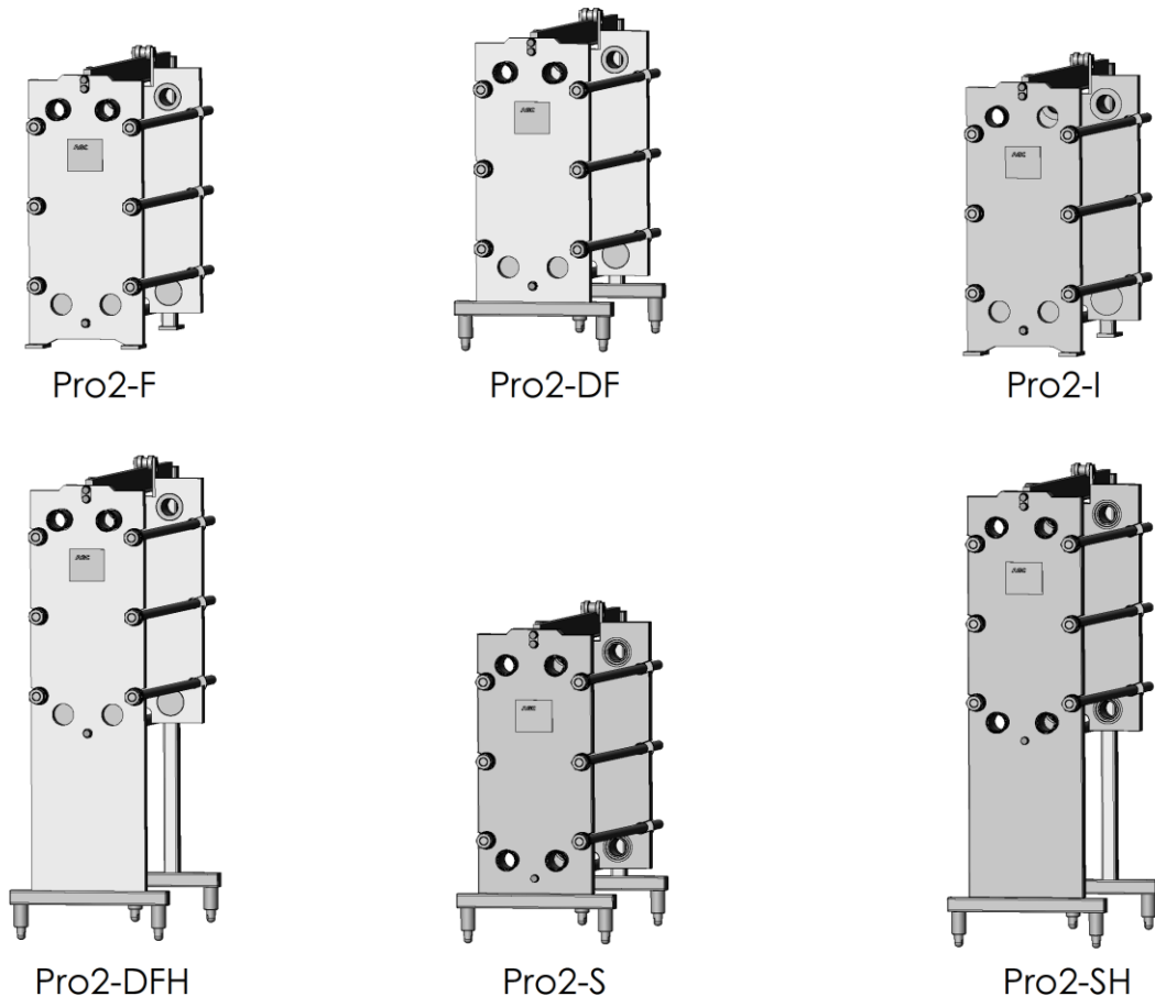
Figure 9 Pro2 Tiebolt Frame Assemblies
