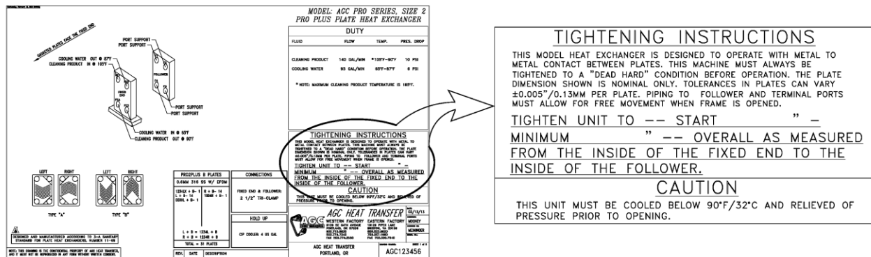
Figure 7 Tightening Instructions
