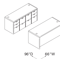
MODULAR DESK AND CREDEZA 66" W x 96" D
