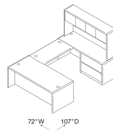
DESK "U" WORKSTATION – RIGHT 72"W x 107"D
