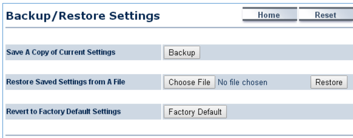
Figure 5-51 Backup/Restore Settings
