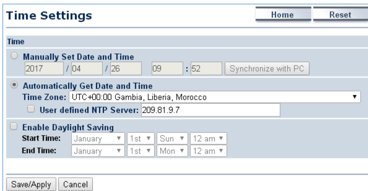
Figure 5-54 Time Settings
