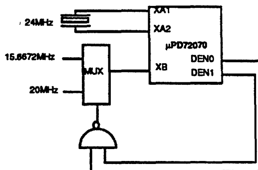
Recommended Circuit #2
