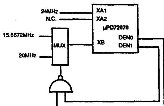
Recommended Circuit #1
