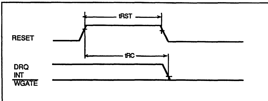
Fig.5 Reset Timing
