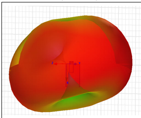
FIGURE 7-3: 3D RADIATION PATTERN AND ANTENNA ORIENTATION
