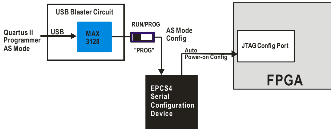
Figure 4.2. The AS configuration scheme.
