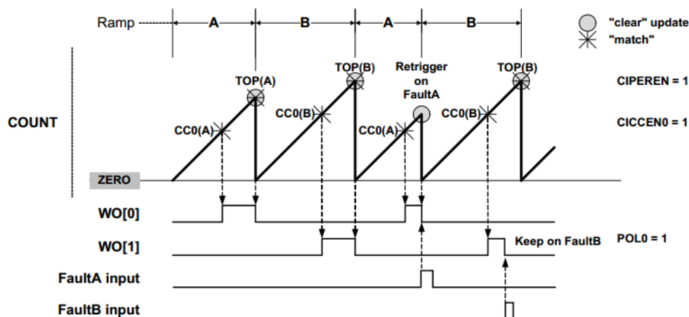
Figure 5-15. RAMP2A Operation
