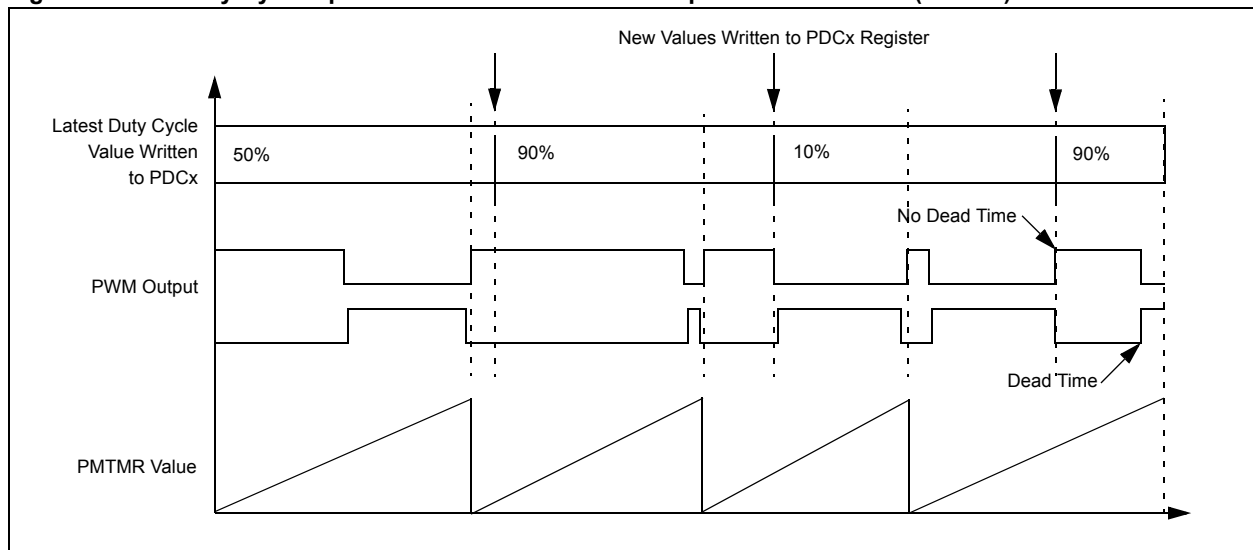
Figure 14-82: Duty Cycle Update Times When Immediate Updates are Enabled (IUE = 1)
