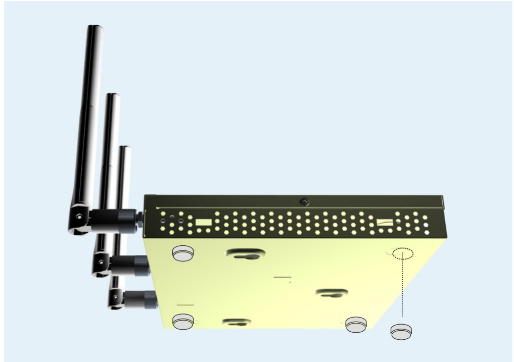
Figure 10: Attach Feet
