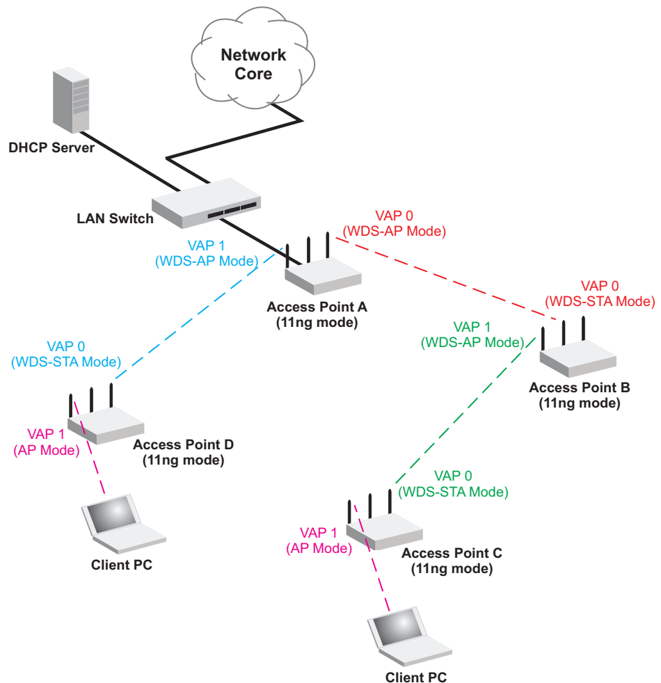
Figure 66: WDS Links Between Three or More APs
