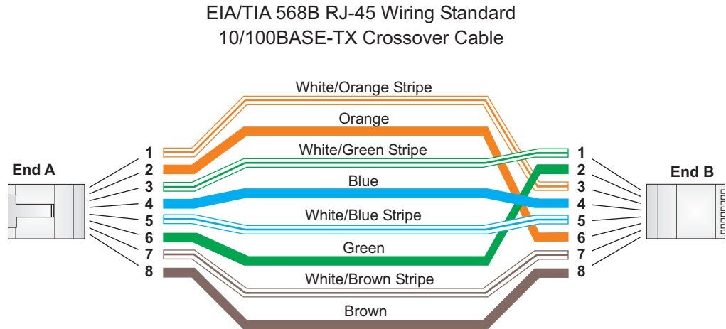
Figure 69: Crossover Wiring
