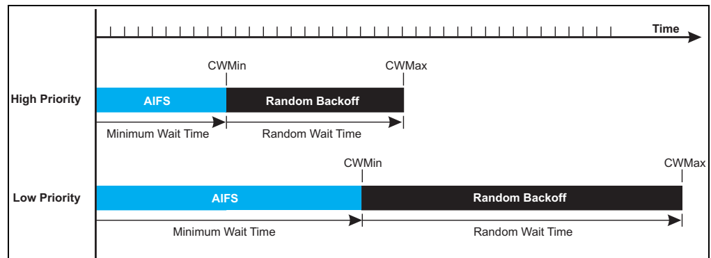
Figure 49: WMM Backoff Wait Times
