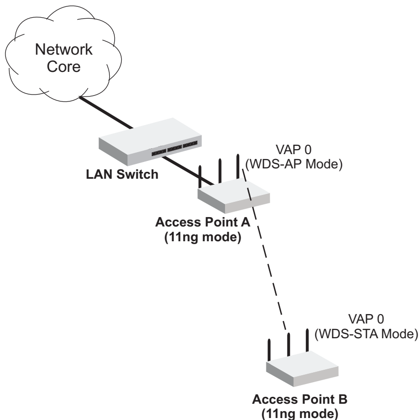
Figure 58: Basic WDS Link Between Two APs
