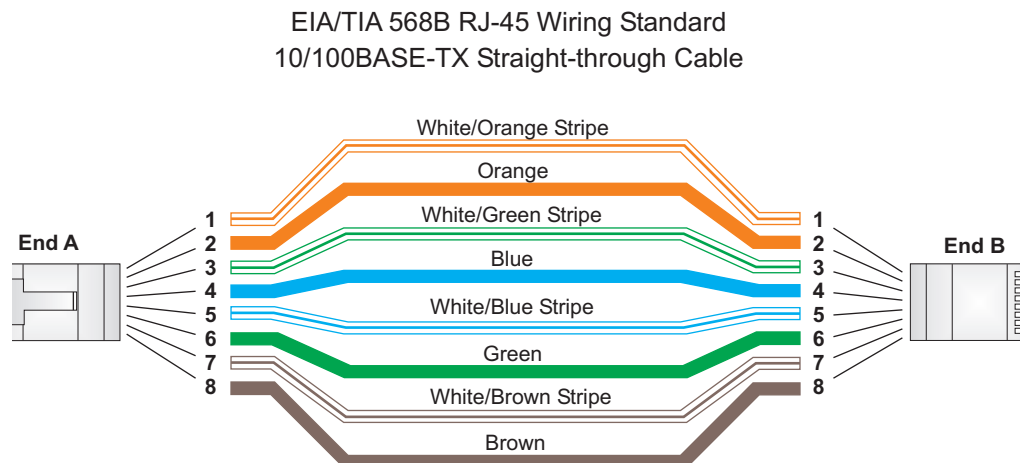
Figure 68: Straight Through Wiring
