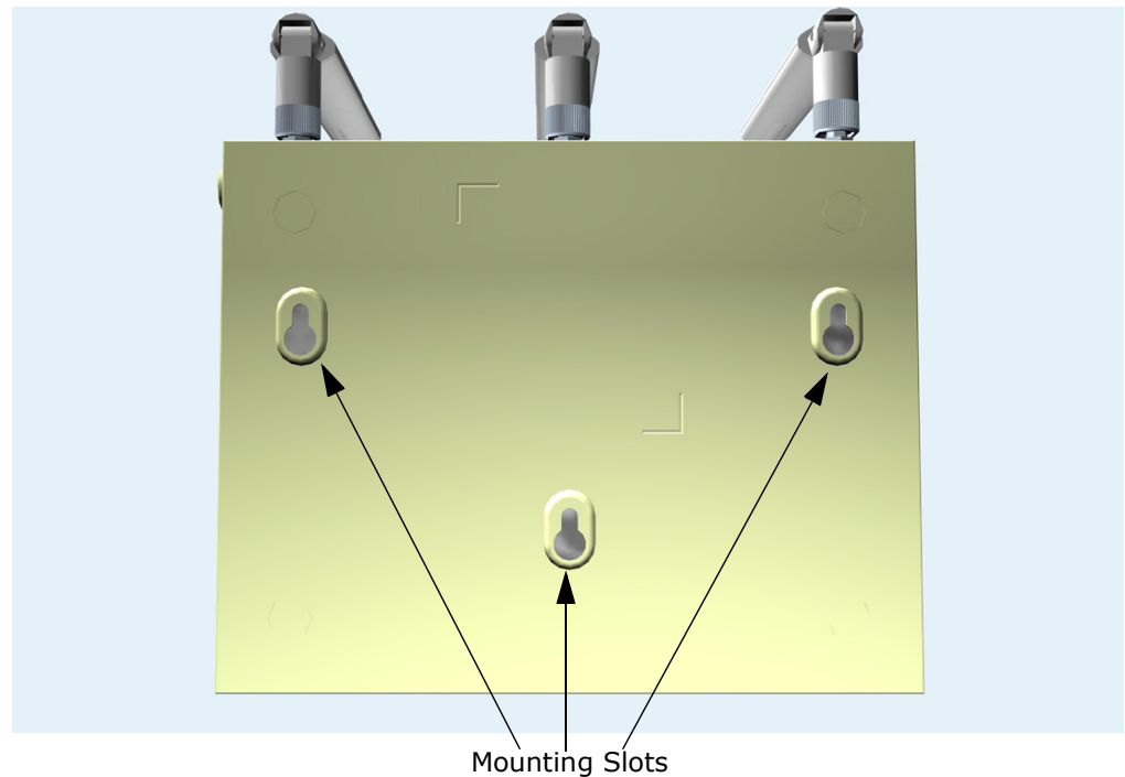
Figure 11: Wall Mounting
