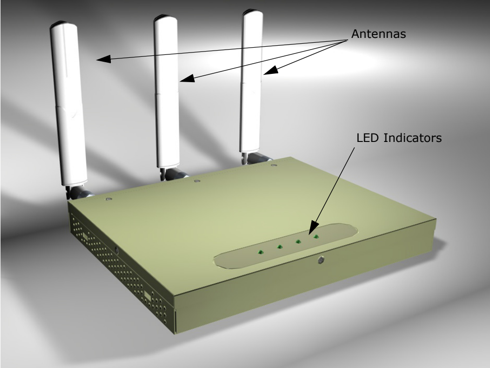
Figure 1: Top Panel
