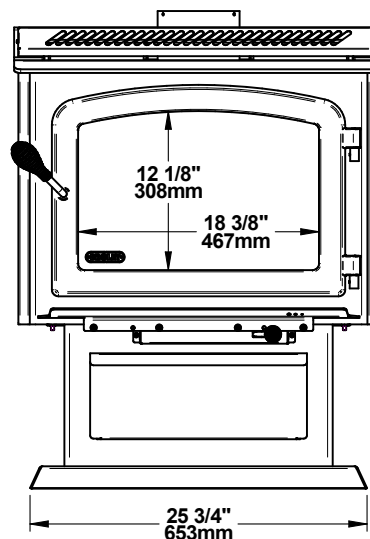
Figure 2: Front view
