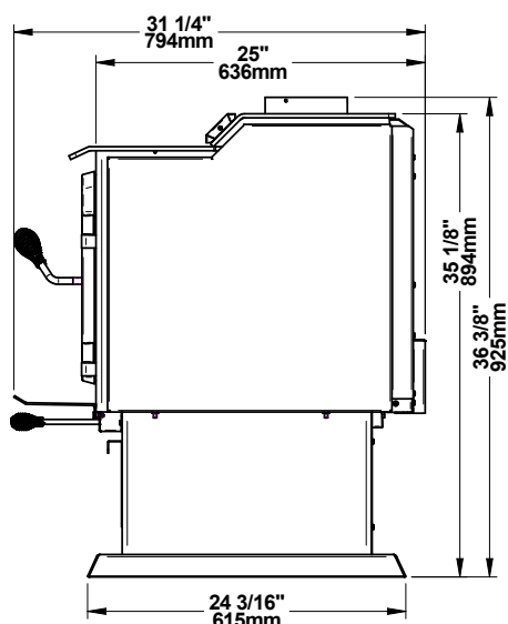
Figure 3: Side view
