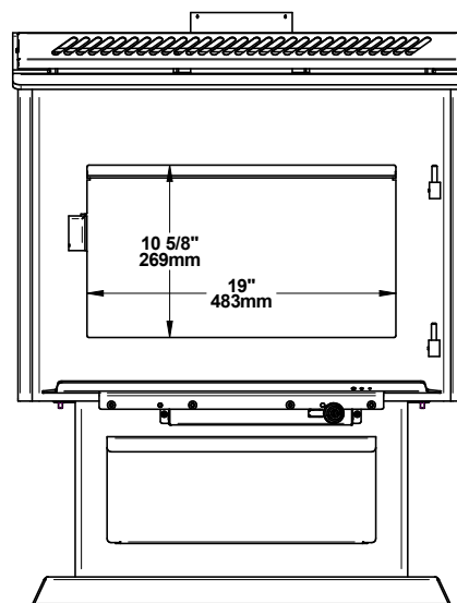
Figure 6: Door opening
