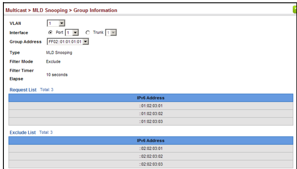
Figure 364: Showing IPv6 Multicast Services and Corresponding Sources
