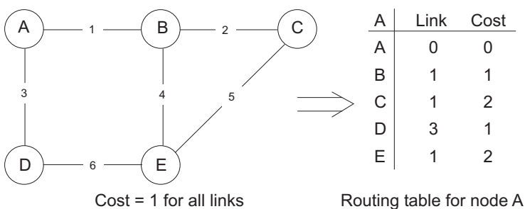
Figure 432: Configuring RIP
