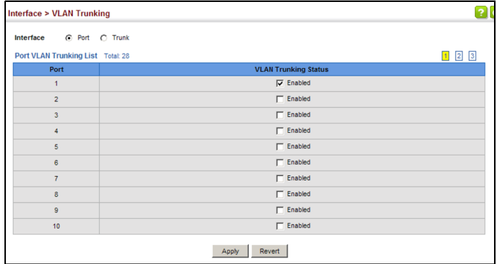
Figure 68: Configuring VLAN Trunking
