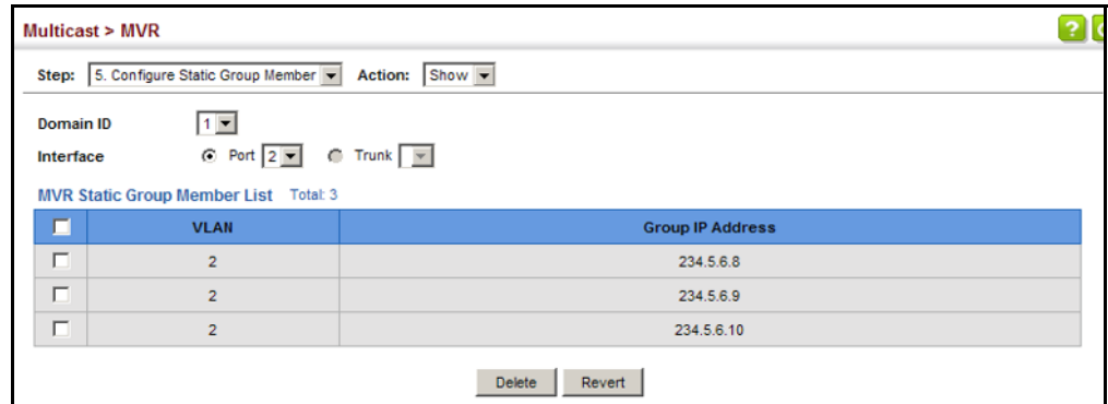
Figure 374: Showing the Static MVR Groups Assigned to a Port
