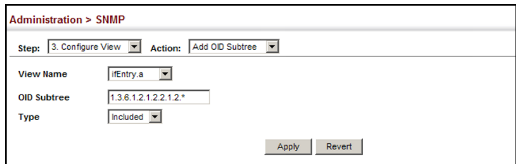
Figure 260: Adding an OID Subtree to an SNMP View
