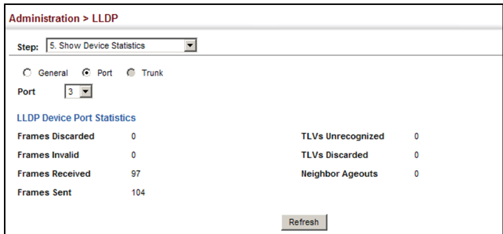
Figure 252: Displaying LLDP Device Statistics (Port)
