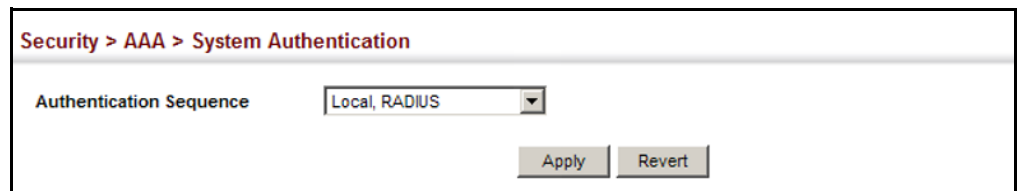
Figure 158: Configuring the Authentication Sequence
