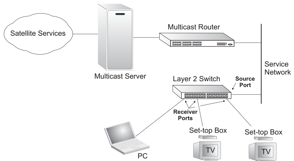
Figure 365: MVR Concept
