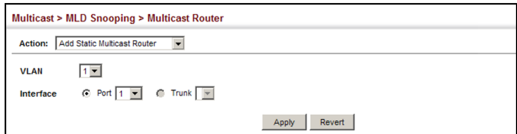
Figure 358: Configuring a Static Interface for an IPv6 Multicast Router
