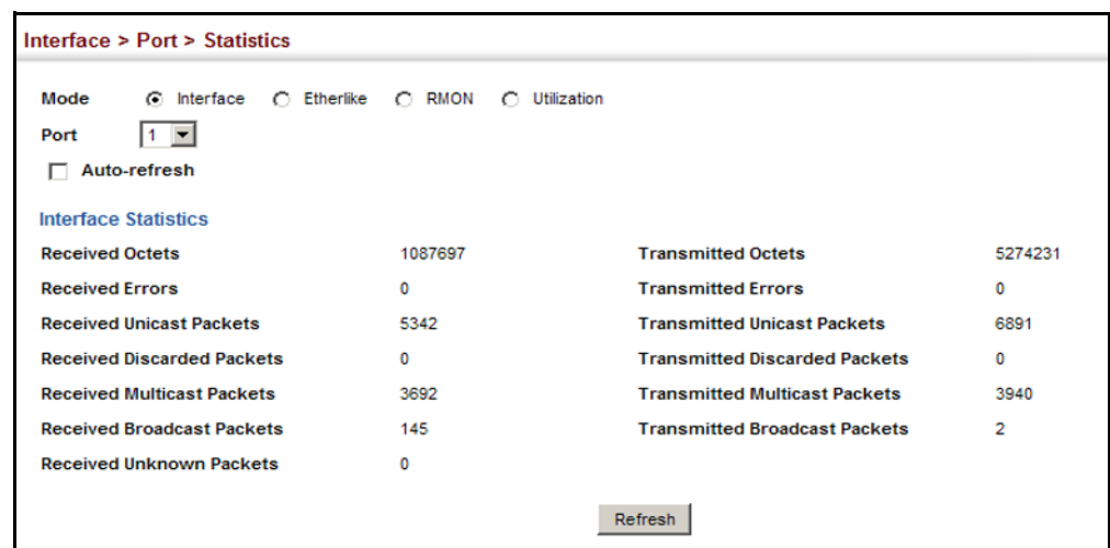
Figure 42: Showing Port Statistics (Table)
