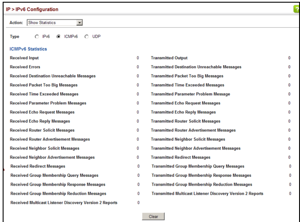
Figure 402: Showing IPv6 Statistics (ICMPv6)
