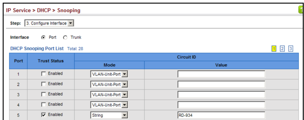
Figure 235: Configuring the Port Mode for DHCP Snooping
