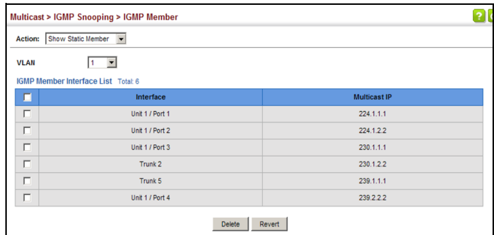
Figure 342: Showing Static Interfaces Assigned to a Multicast Service
