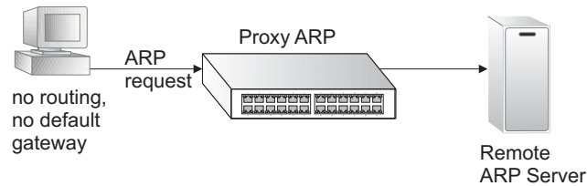
Figure 423: Proxy ARP
