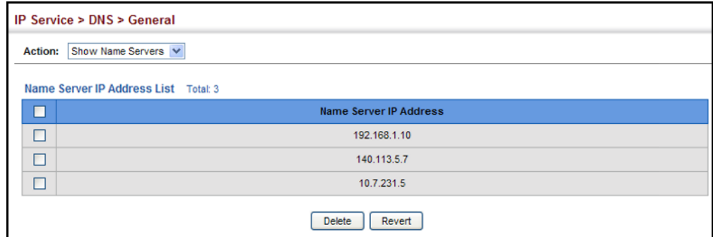
Figure 409: Showing the List of Name Servers for DNS
