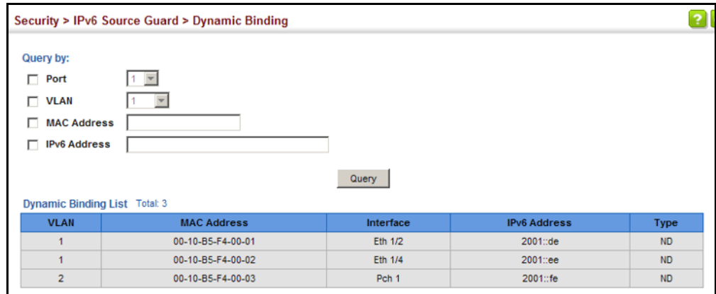
Figure 232: Showing the IPv6 Source Guard Binding Table
