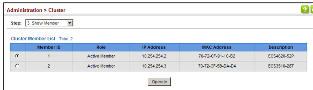
Figure 291: Managing a Cluster Member
