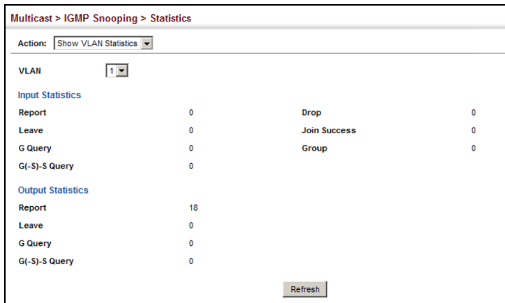
Figure 348: Displaying IGMP Snooping Statistics – VLAN
