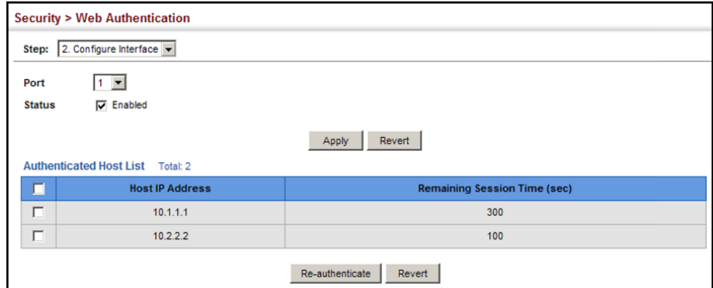
Figure 179: Configuring Interface Settings for Web Authentication
