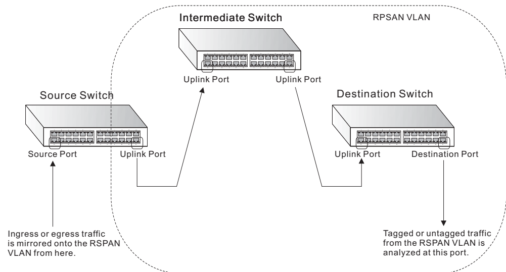
Figure 38: Configuring Remote Port Mirroring
