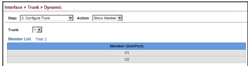
Figure 56: Showing Members of a Dynamic Trunk
