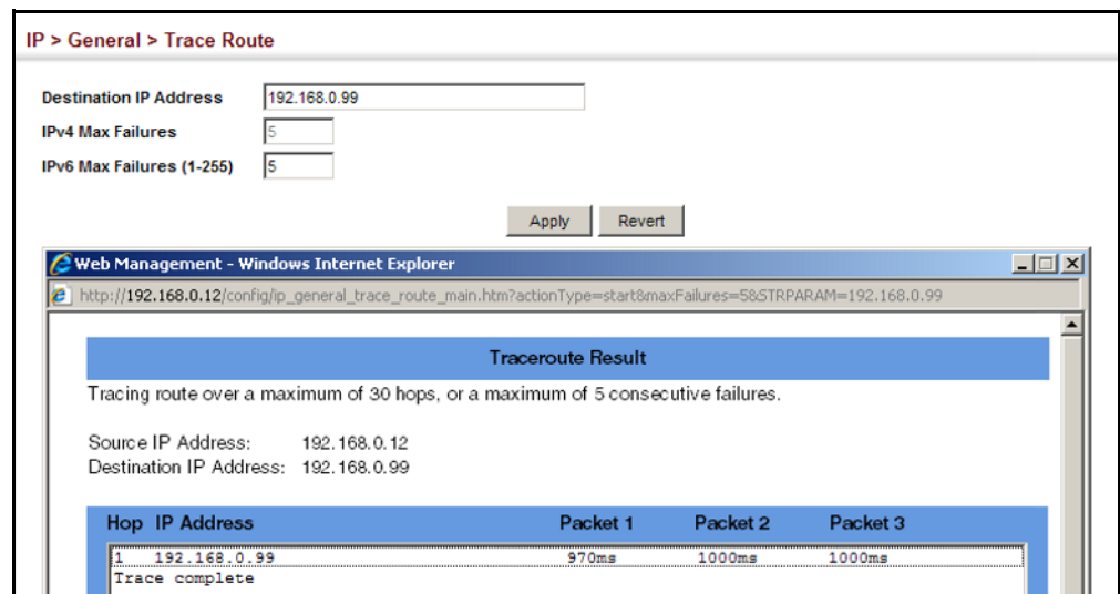
Figure 422: Tracing the Route to a Network Device
