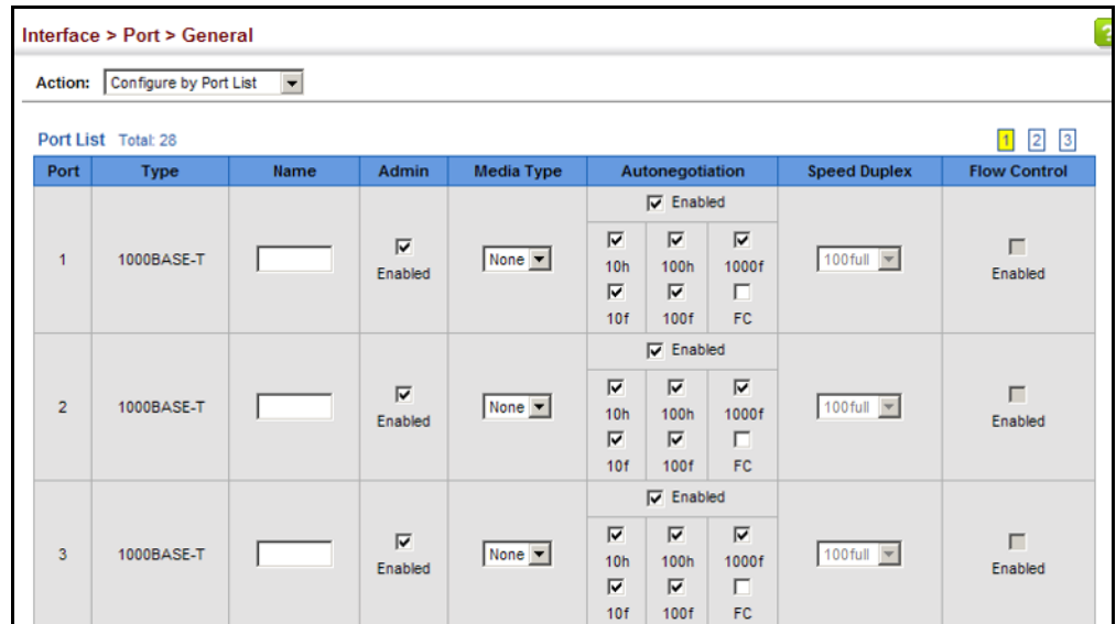
Figure 32: Configuring Connections by Port List
