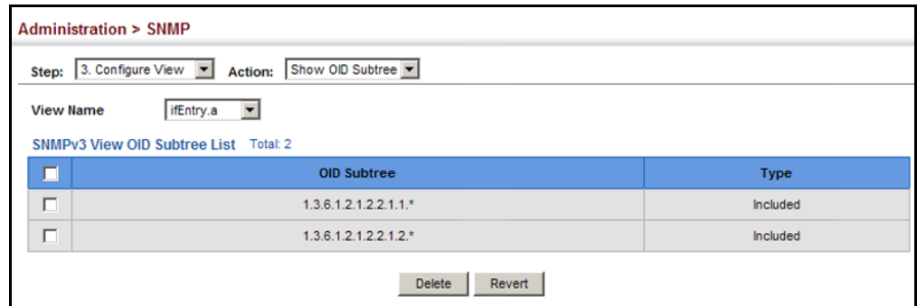
Figure 261: Showing the OID Subtree Configured for SNMP Views
