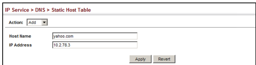
Figure 410: Configuring Static Entries in the DNS Table
