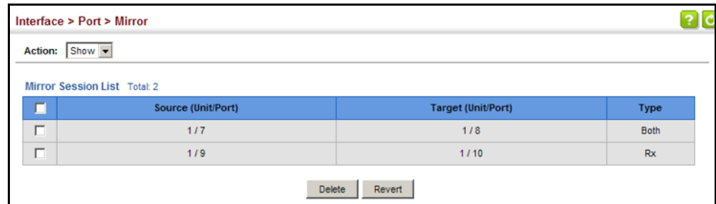
Figure 37: Displaying Local Port Mirror Sessions
