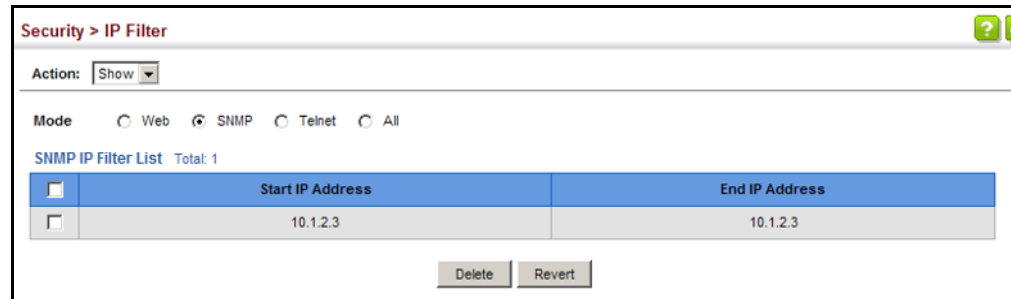
Figure 216: Showing IP Addresses Authorized for Management Access
