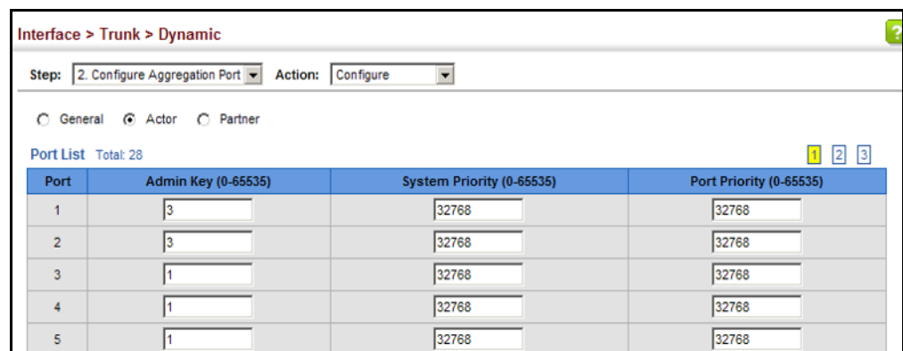
Figure 55: Configuring LACP Parameters on a Port
