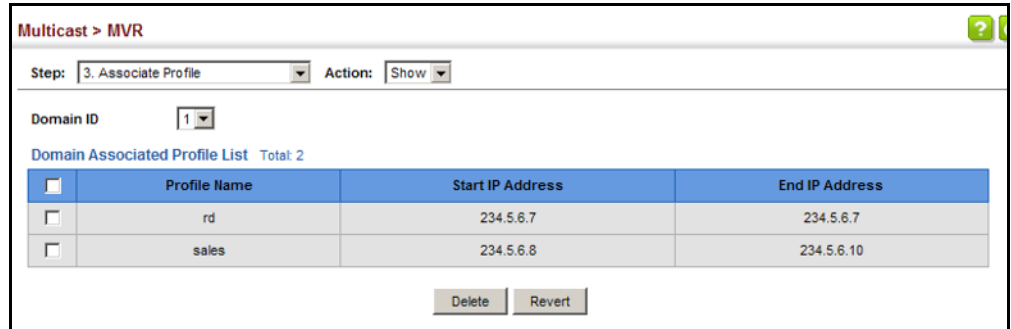
Figure 371: Showing the MVR Group Address Profiles Assigned to a Domain
