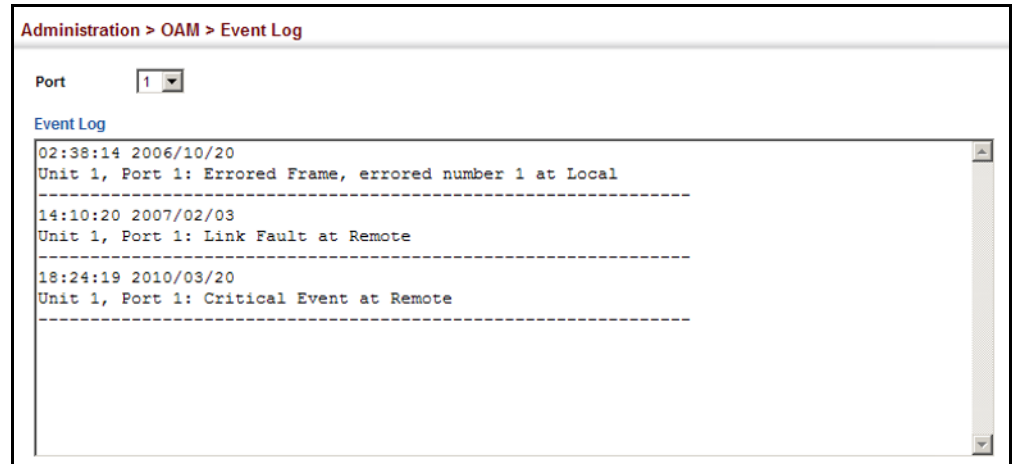
Figure 329: Displaying the OAM Event Log
