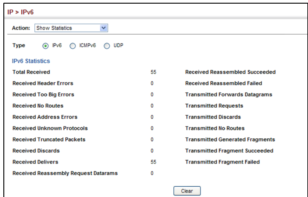
Figure 401: Showing IPv6 Statistics (IPv6)
