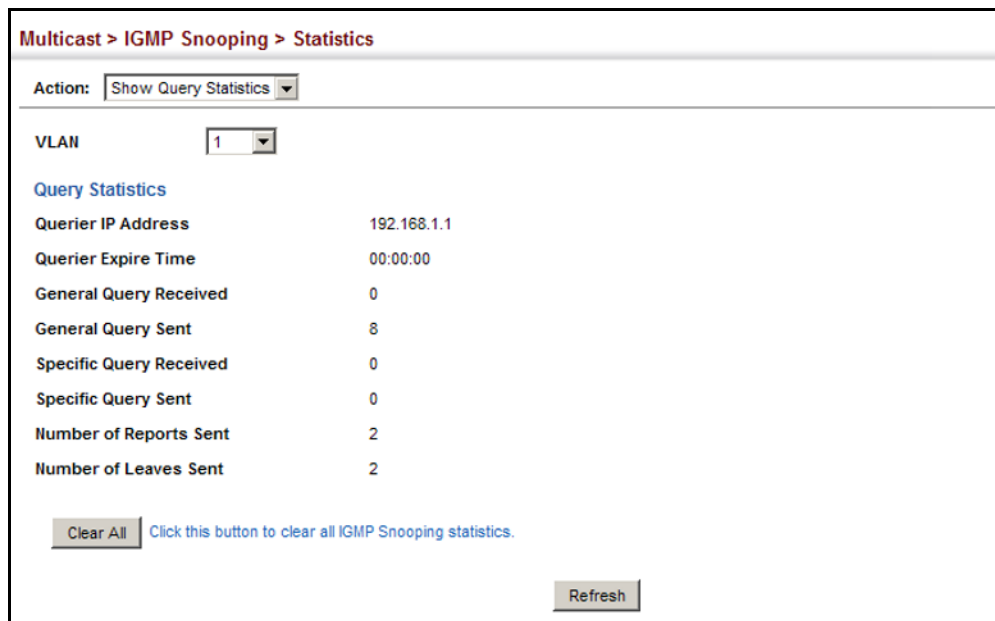
Figure 347: Displaying IGMP Snooping Statistics – Query
