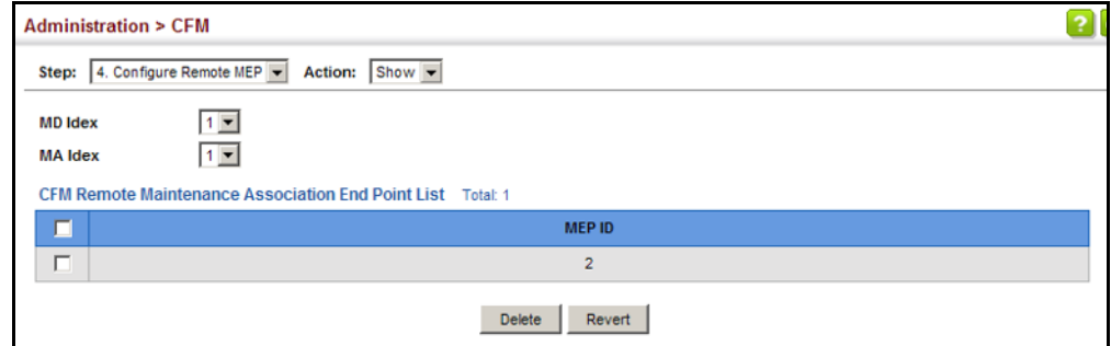
Figure 315: Showing Remote Maintenance End Points
