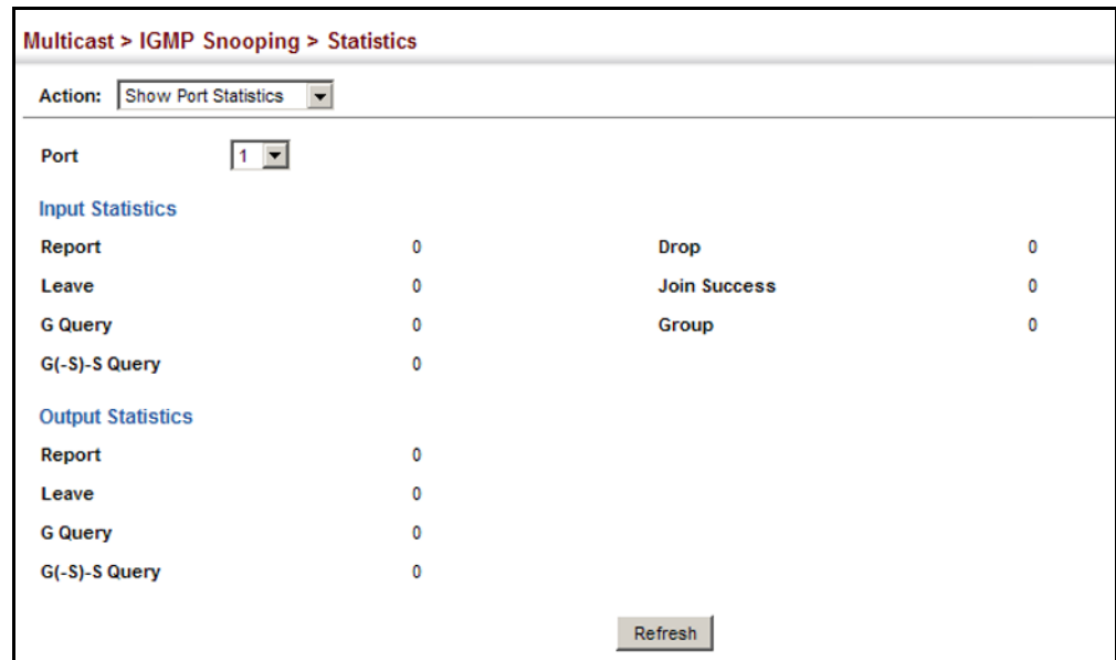
Figure 349: Displaying IGMP Snooping Statistics – Port
