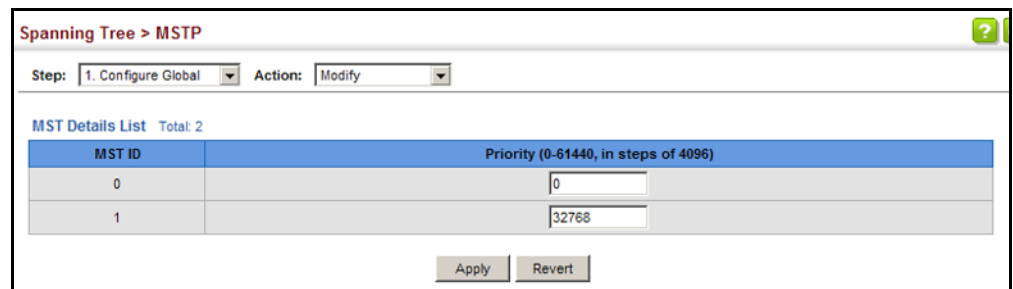
Figure 122: Modifying the Priority for an MST Instance
