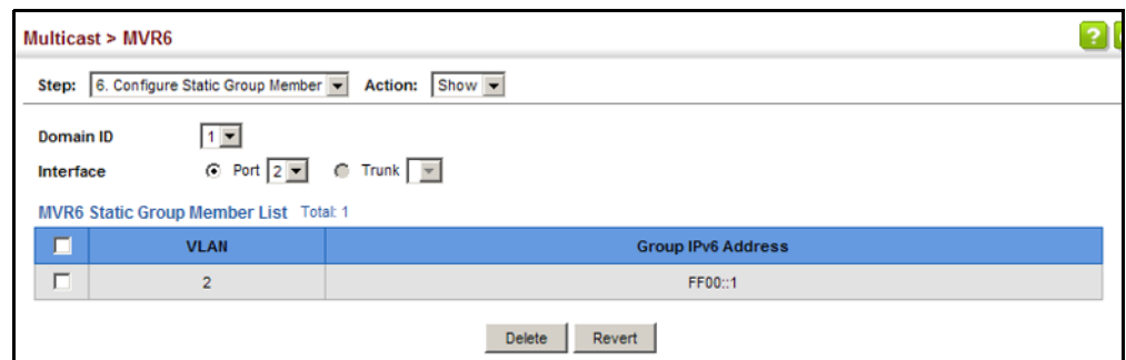
Figure 387: Showing the Static MVR6 Groups Assigned to a Port
