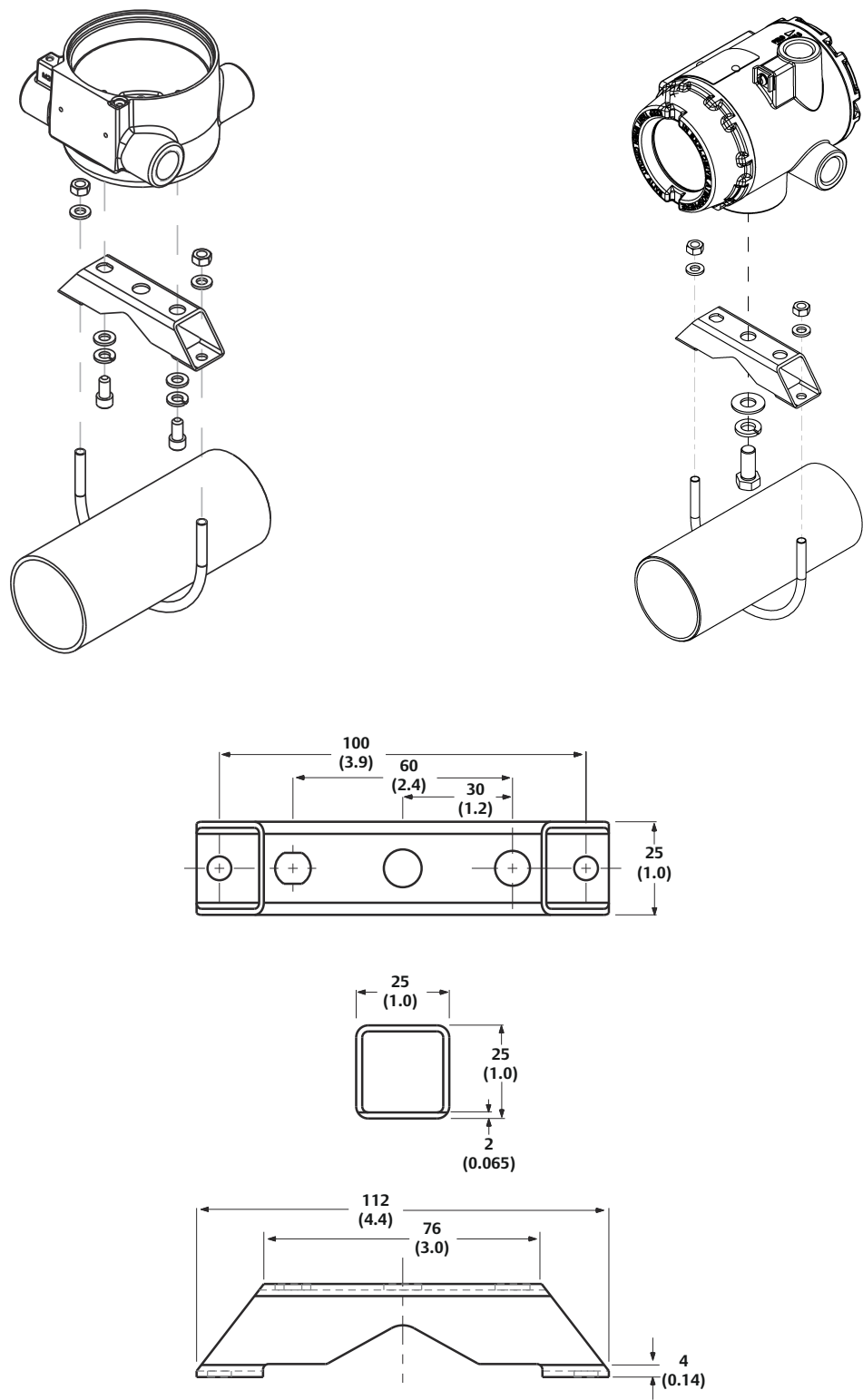
Figure 13: Optional Mounting
