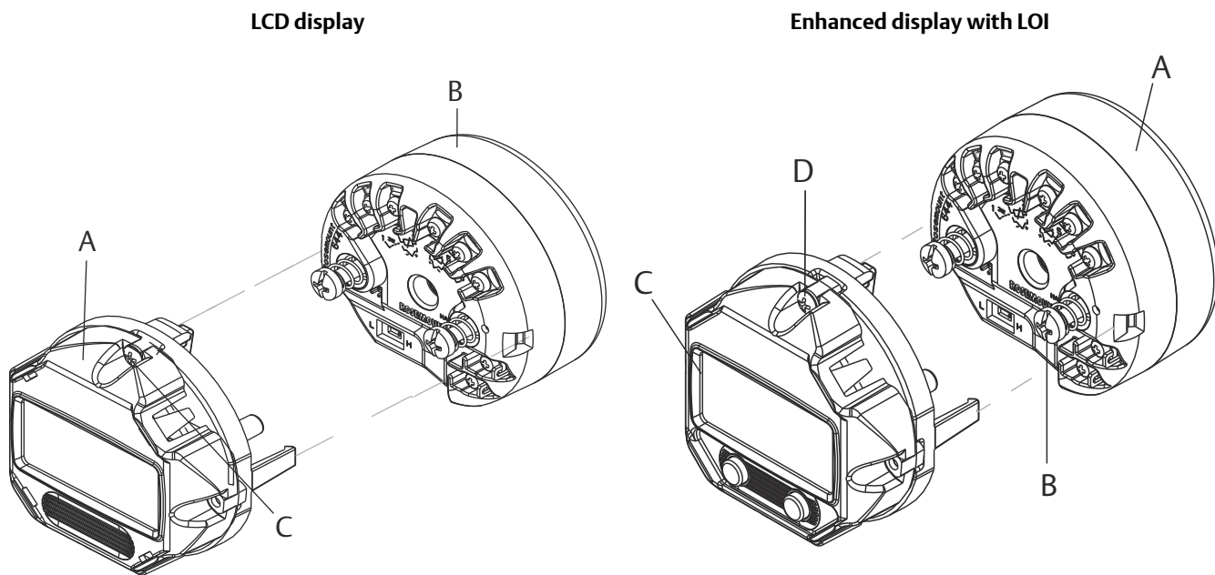
Figure 12: Display
