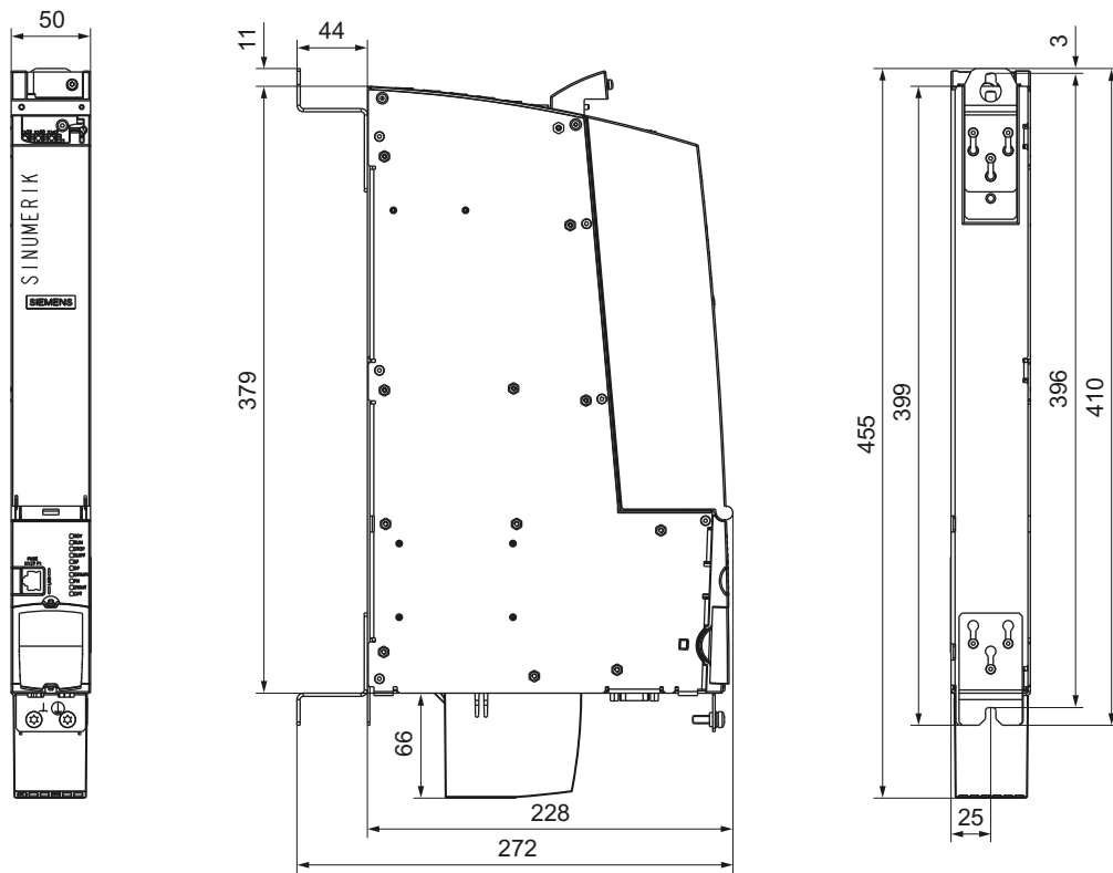
Figure 5-2 Dimension drawing NCU 710.3 PN; dimensions in mm
