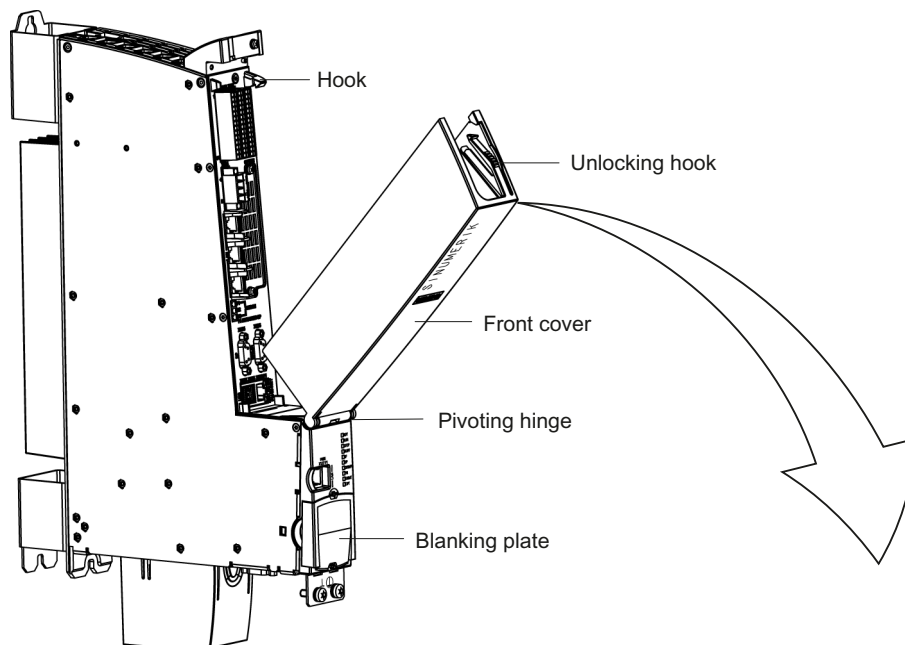
Figure 7-2 Removing the front cover
