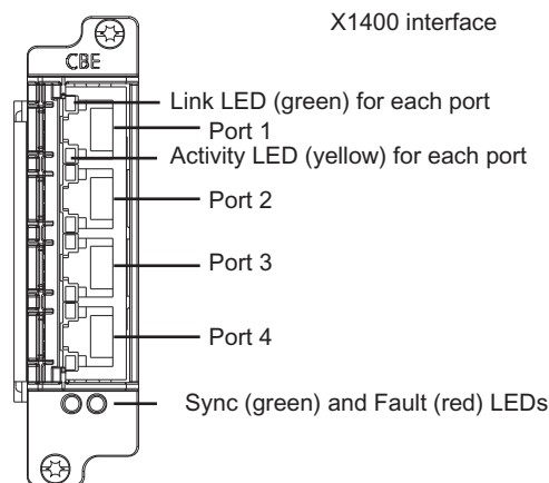
Figure 9-23 CBE30-2 Ethernet communication board
