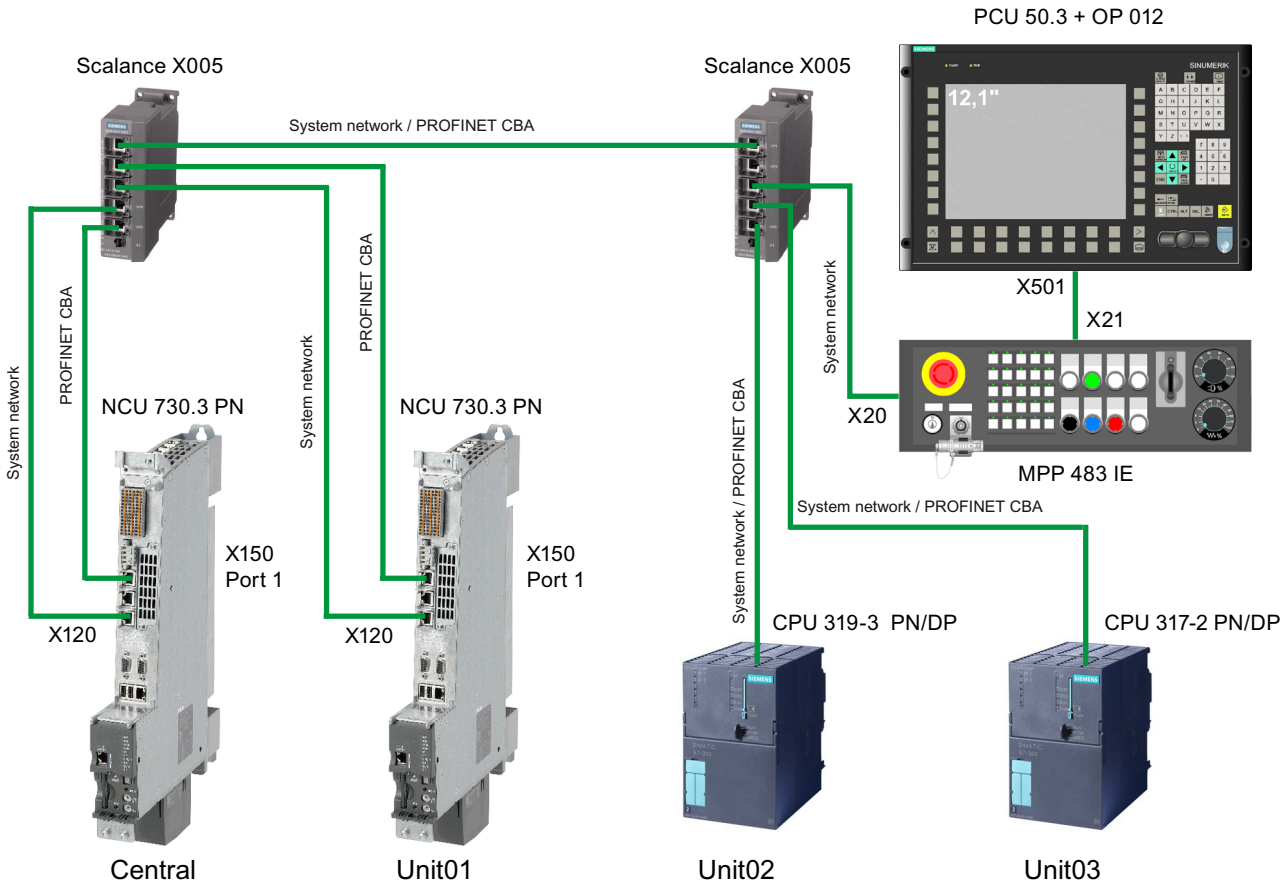
Figure 7-8 Example PROFINET CBA configuration
