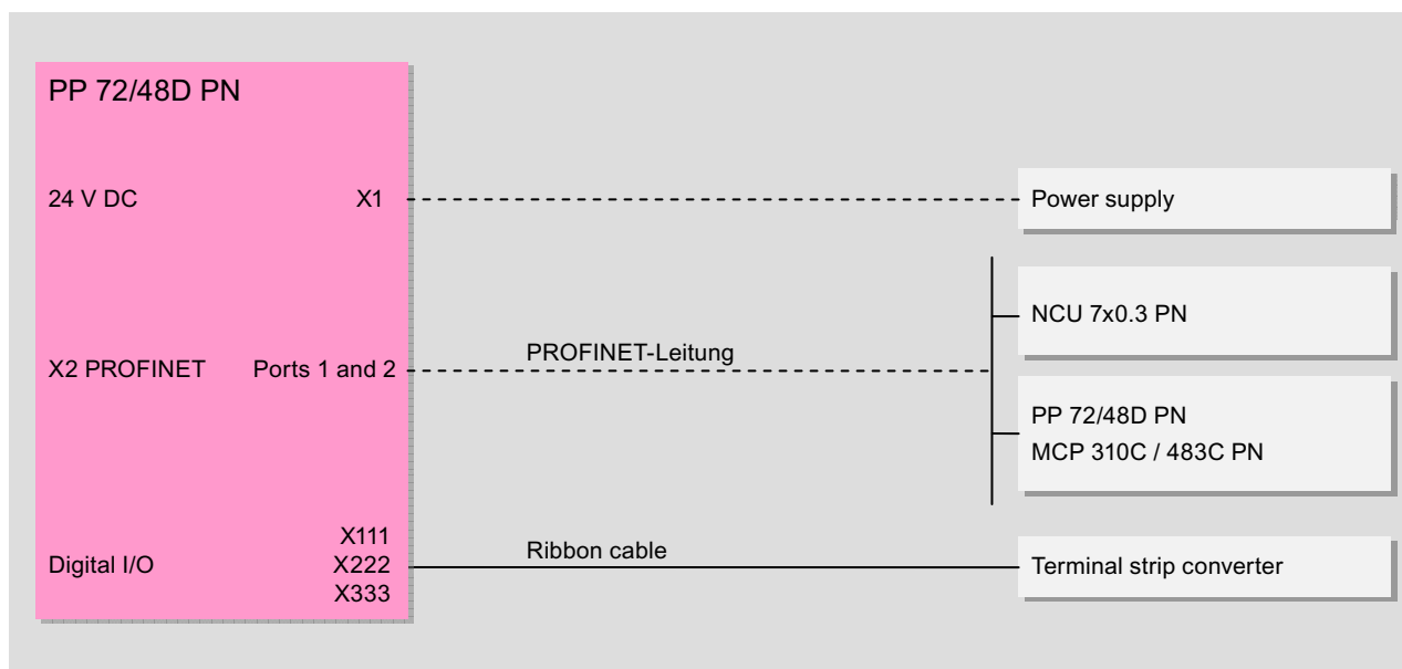
Figure 9-10 I/O module connection options
