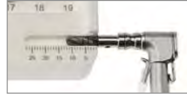
Measure With Drill Stop Attached To Confirm Desired Drill Depth
