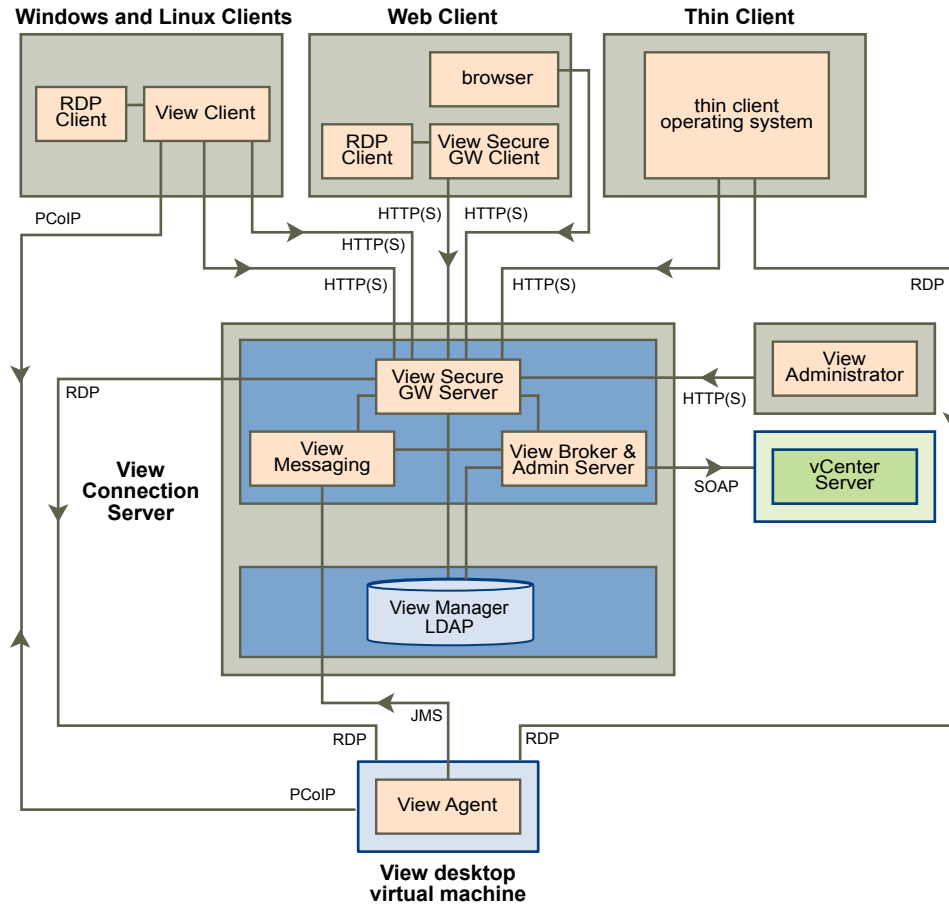
Figure 5-5. VMware View Components and Protocols without a Security Server
