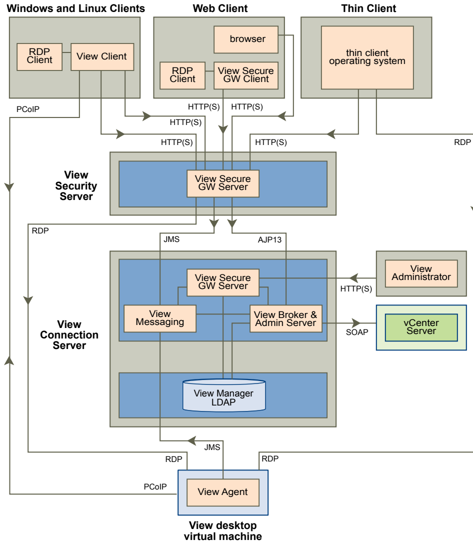
Figure 5-6. VMware View Components and Protocols with a Security Server
