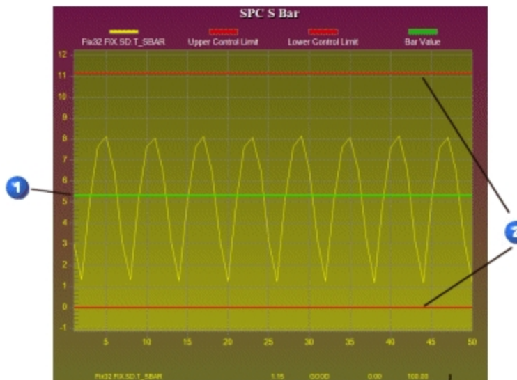
S-Bar Chart
