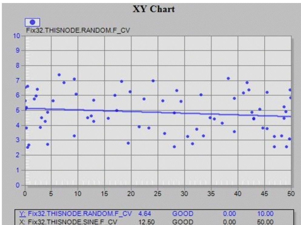
XY Chart
