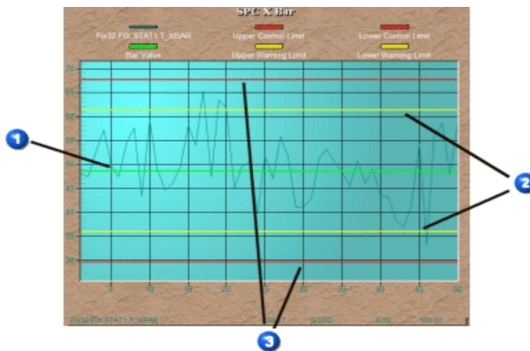
X-Bar Chart
