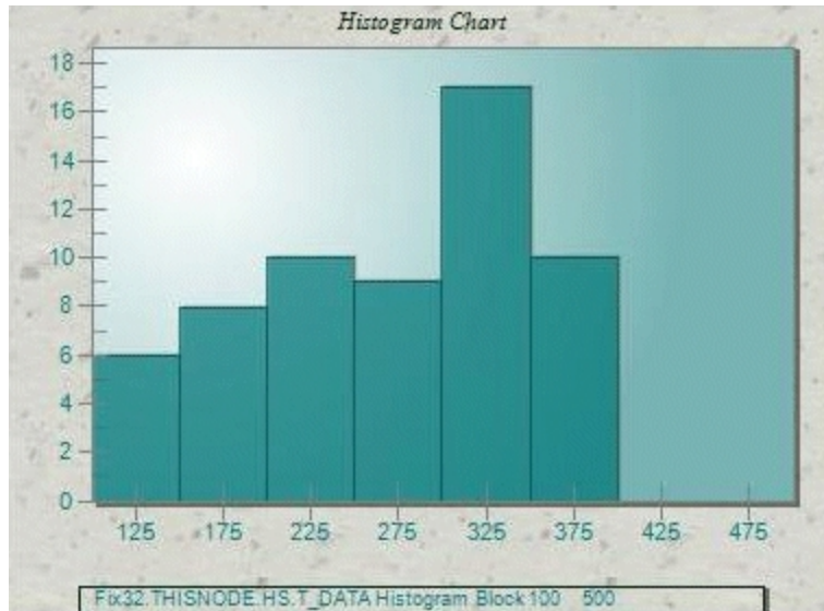
Histogram Chart
