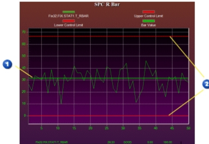
R-Bar Chart
