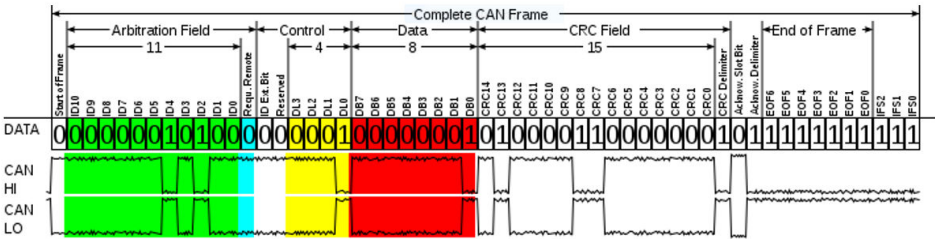
Figure 80. Base frame format
