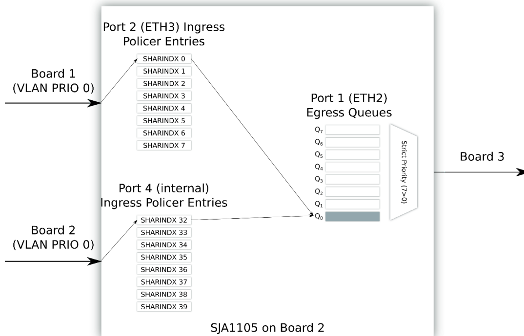
Figure 47. Queuing diagram
