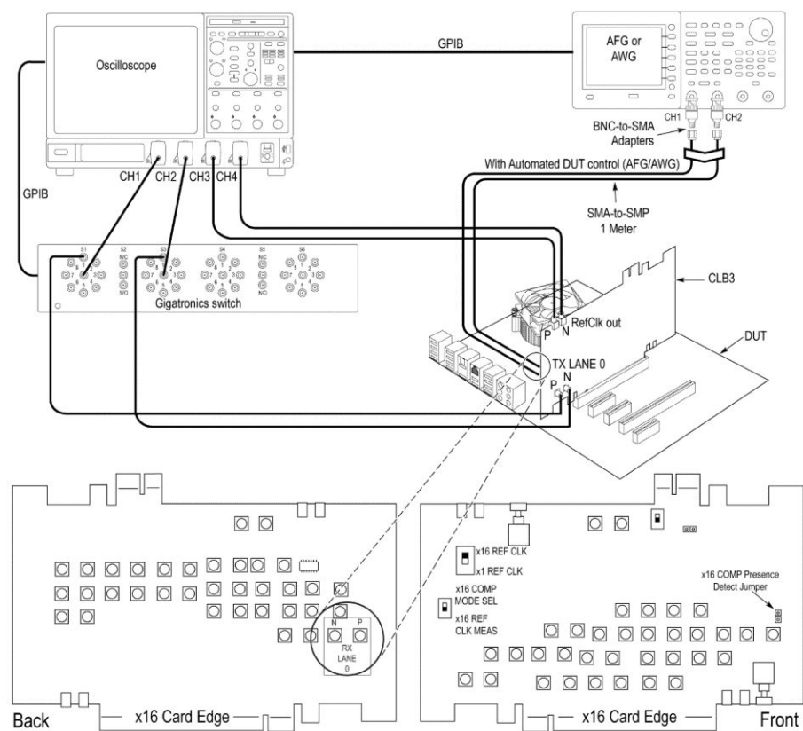
Figure 4: System board (normal) connection setup through switch system
