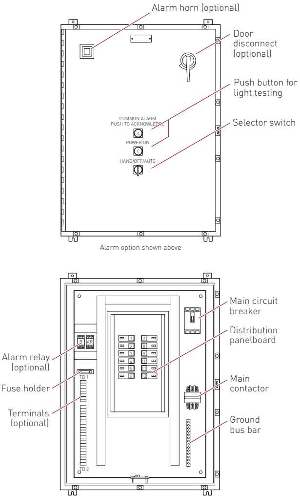
Figure 28: HTPG power distribution panel
