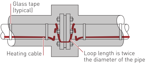
Figure 11: Flange
