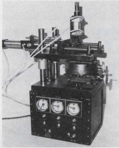
Aremco's 1975 version of its 3100 screen printer provides new squeegee pressure controls, settable timers, vibration-free motion and 0.0003-in. repeatability.
