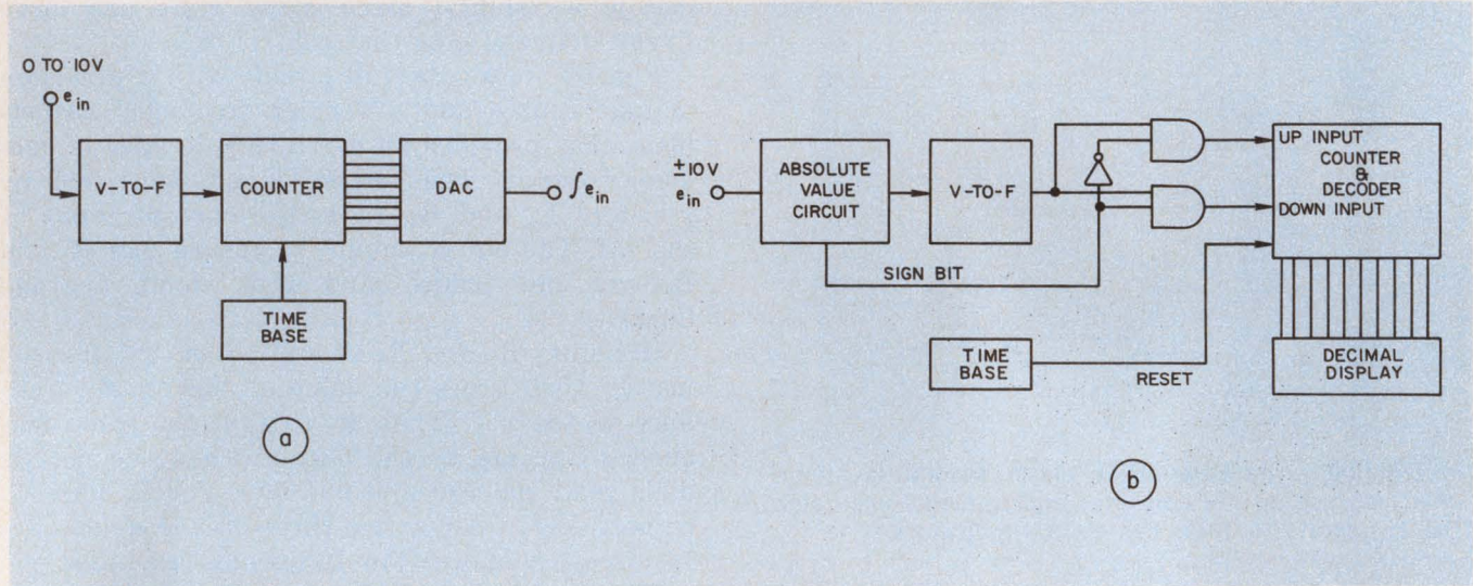
7. A v/f converter combined with a counter, time base and d/a converter makes a simple integrator (a). By eliminating the d/a and using an up/down counter, you can build a simple integrating digital voltmeter (b).
