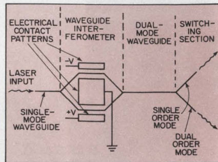
Modulating and switching device, which uses micro-optics, is said to be easier to fabricate than an equivalent optical IC.
