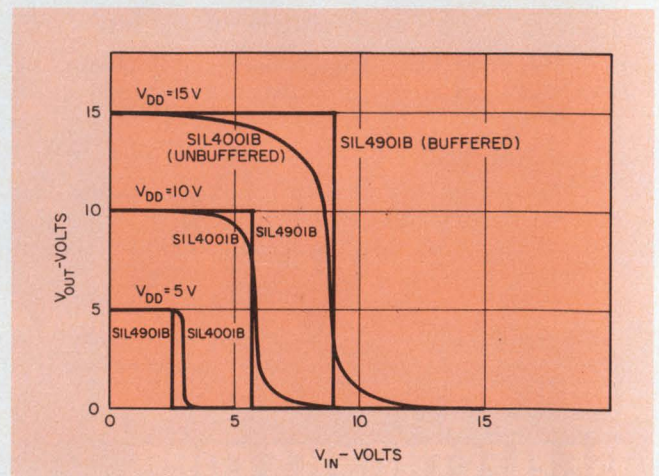
2. Nearly ideal transfer characteristics are offered by buffered gates. Hence they provide higher noise immunity than unbuffered circuits.
