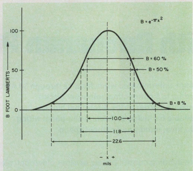
1. Brightness distribution across the width of a CRT spot or line: If the distribution is gaussian, the width at the 50%-brightness point will be 1.9 times less than the apparent, or perceived, width.
