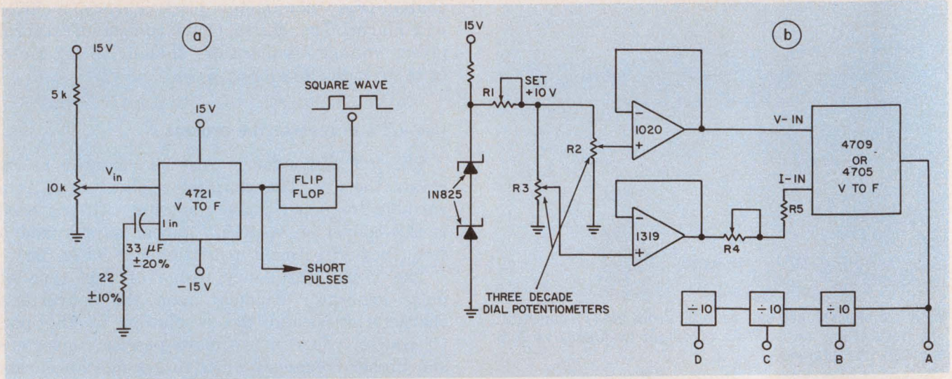
6. Build a simple variable-frequency pulse generator (a) that uses a v/f converter. By modifying the circuit and using decade potentiometers, you can increase the resolution to six decades (b).
