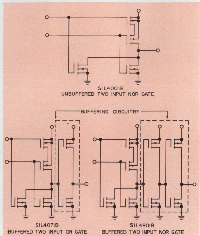
1. Buffered CMOS gates contain a pair of inverters that follow the basic circuit. The inverters isolate the input from the output and provide output drive.
