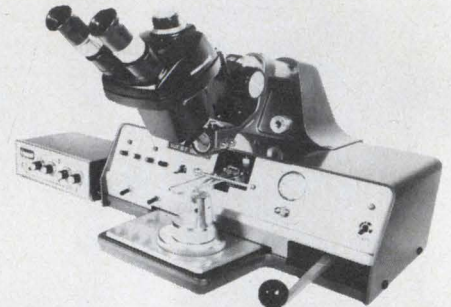
Motorized ultrasonic ball bonders , such as this Model 9700 unit offered by West Bond Equipment, provide the capability of presetting tool motions for repetitive action.
