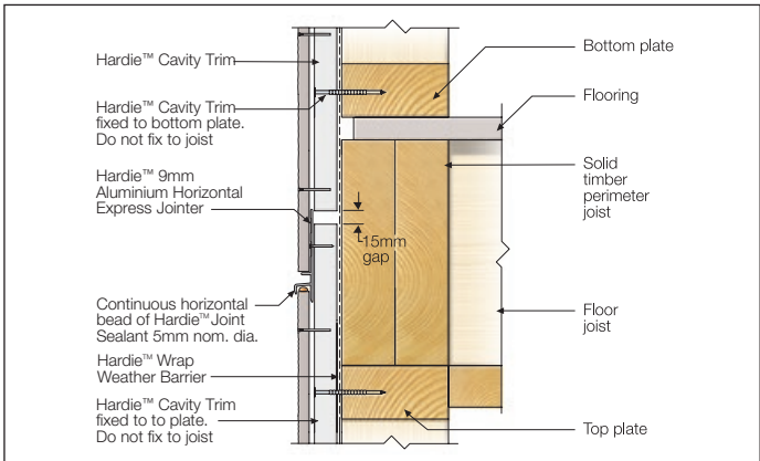
FIGURE 23 FLOOR LEVEL JUNCTION HORIZONTAL EXPRESS JOINDER
