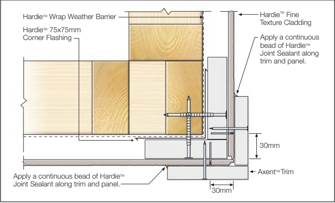
FIGURE 30 TRIM CORNER OPTION - CAVITY TRIM
