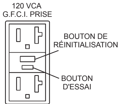
Figure 7. G.F.C.I. Prise
