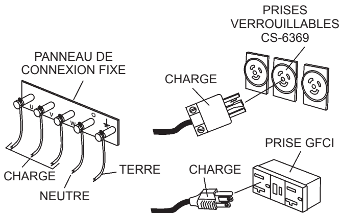
Figure 11. Raccorder les charges
