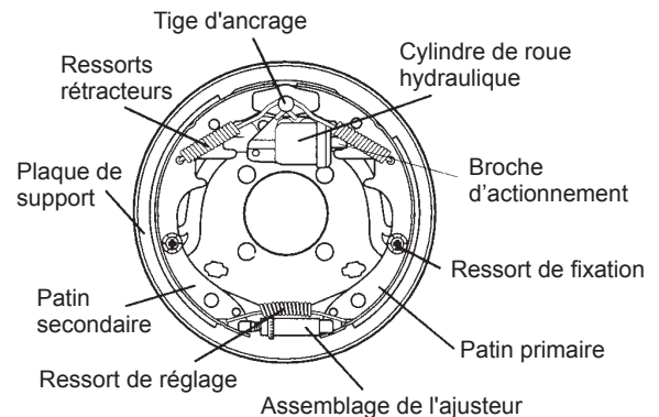
Figure 59. Composants du freinage hydraulique
