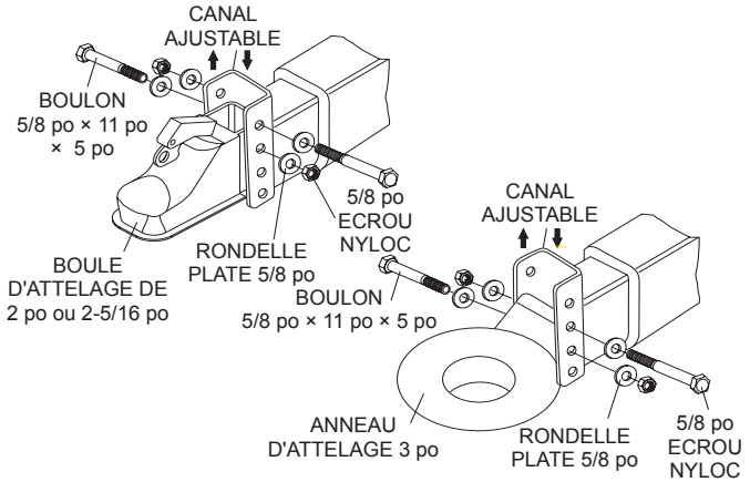
Figure 61. Canal ajustable
