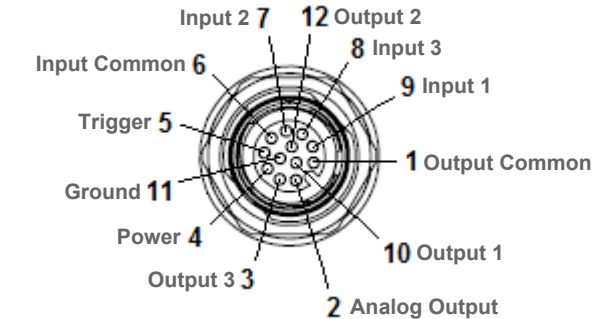
Digital I/O and Power Connector – M12 12-Pin Socket
