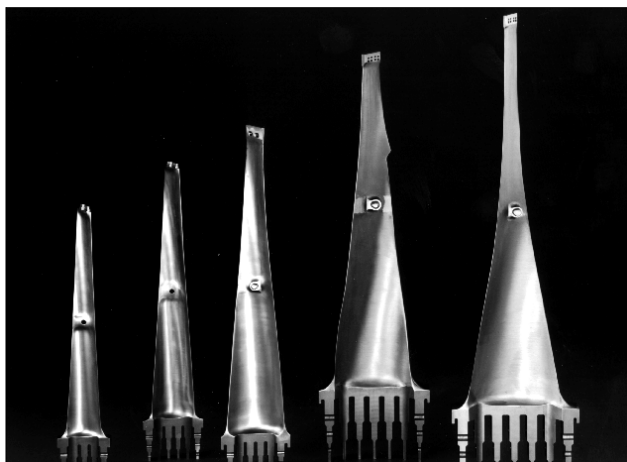
Figure 20. 3600 RPM last-stage bucket family
