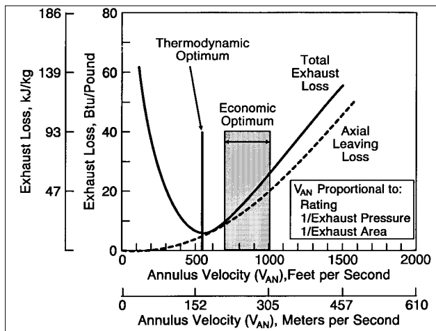
Figure 1. Illustrative exhaust loss curve
