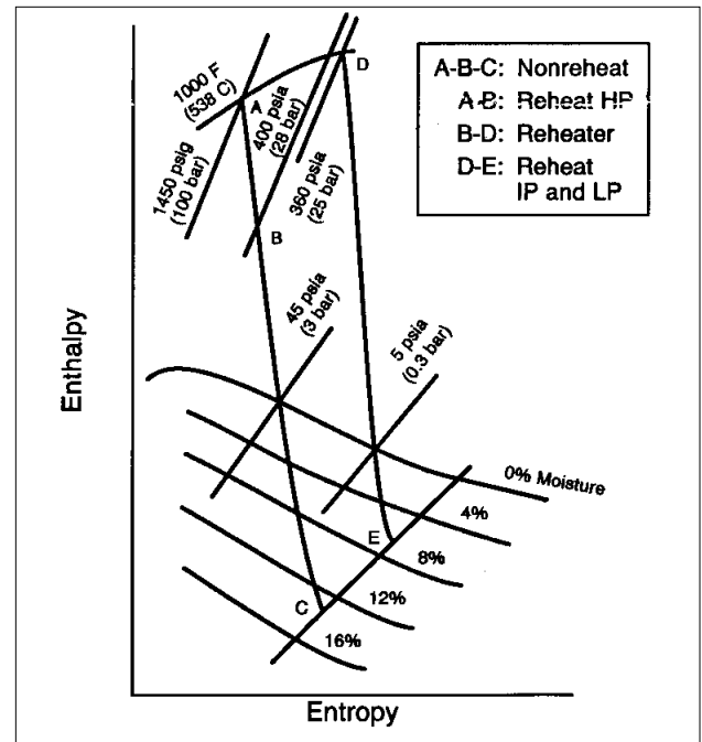
Figure 3. Comparison of nonreheat and reheat expansions
