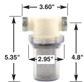
1/2" & 3/4" Strainer
