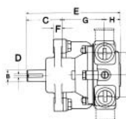
Horizontal Porting G1 &amp; G3
