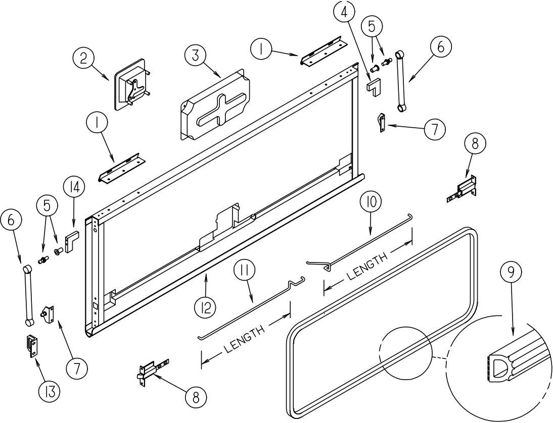
EXTERIOR DOOR COMPONENTS
