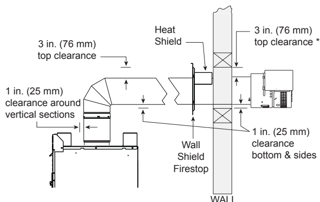
Figure 5.1 Horizontal Venting Clearances To Combustible Materials
