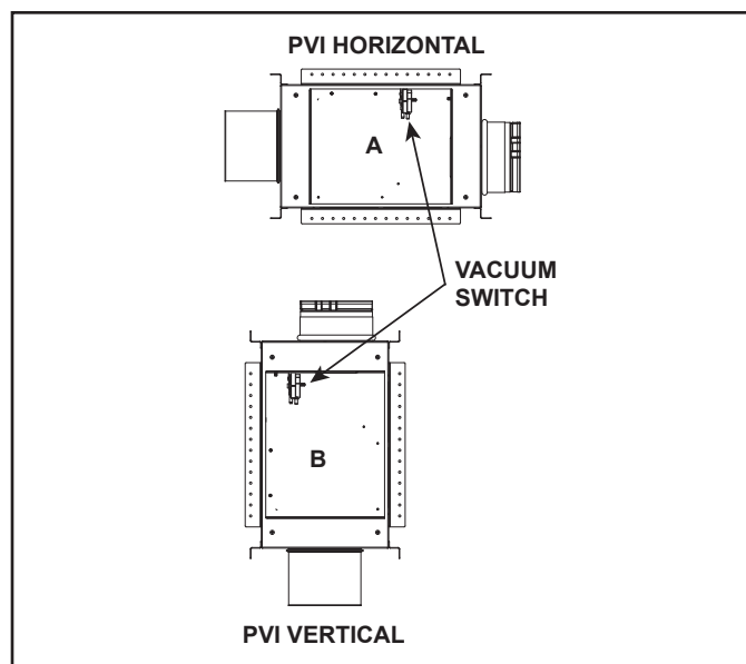
Figure 4.20 Vacuum Switch Location - Horizontal/Vertical Orientation
