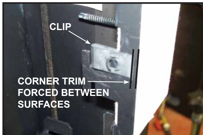
Figure 8. Clip Location.
