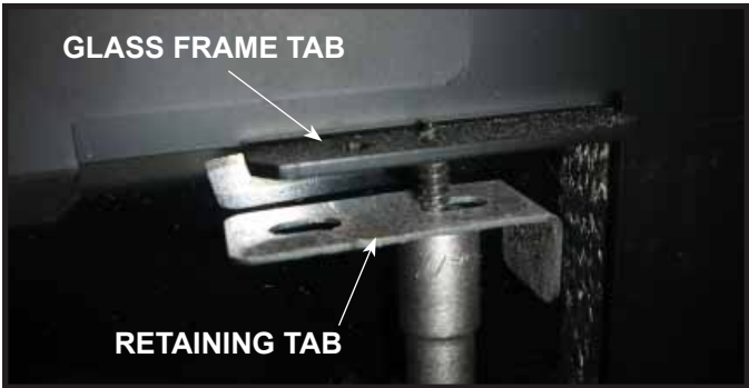
Figure 9. Attaching Retaining Tab to Glass Frame Tab.
