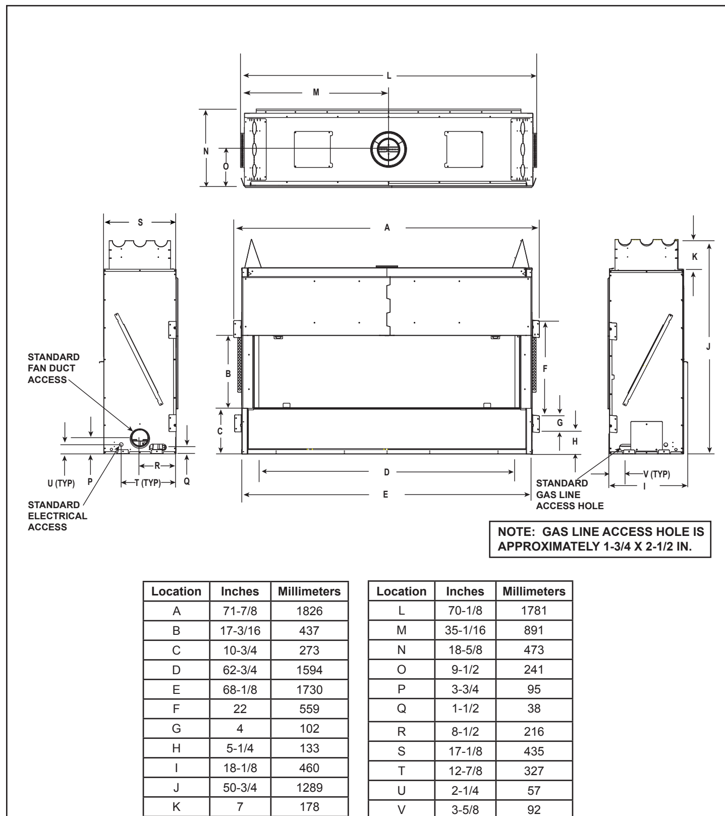
Figure 3.1 Appliance Dimensions
