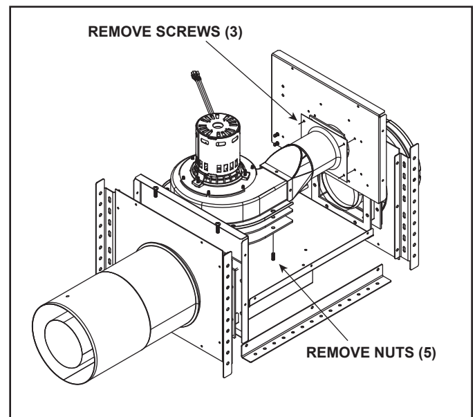
Figure 4.23 Motor Service
