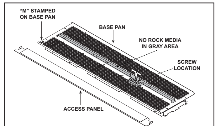
Figure 2. Location of Rock Media Placement Jig
