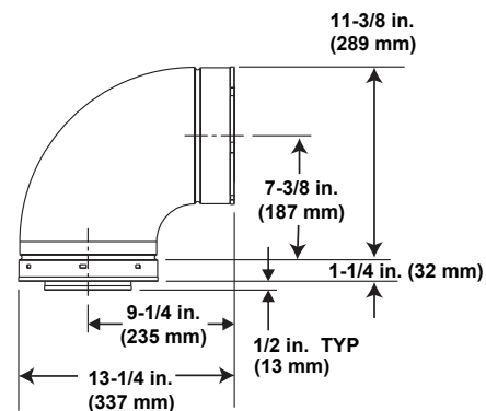
DVP90ST (90° Elbow)
