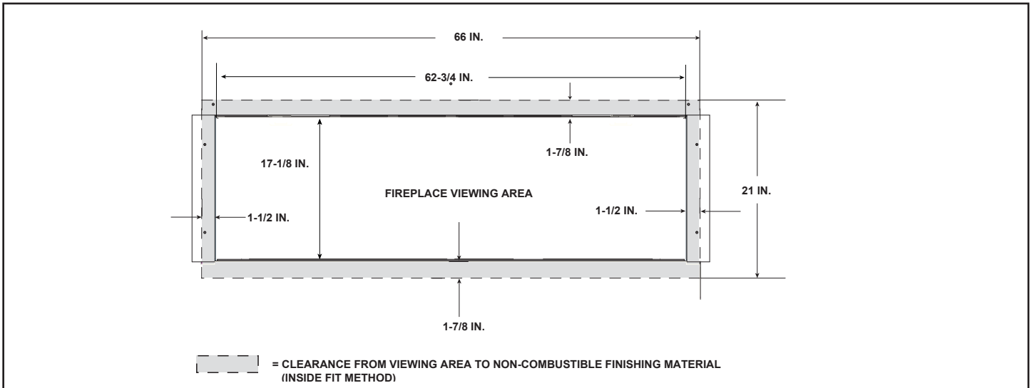
Figure 10.9 Non-Combustible Surface Finishing Material 0-4 Inches Thick-Inside Fit Method
