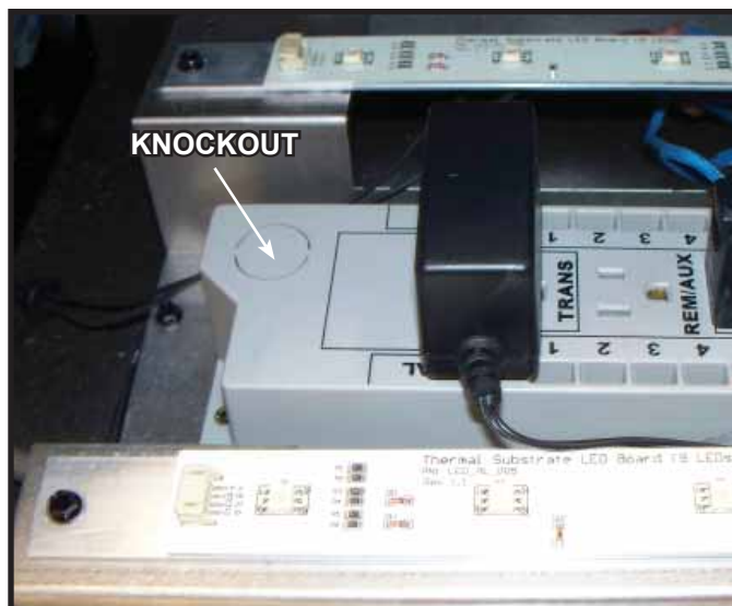
Figure 8.1 Junction Box Detail
