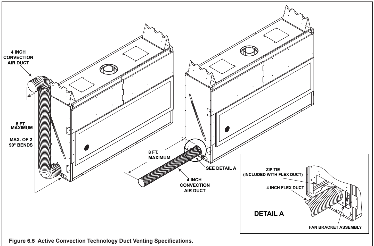
Figure 6.6. Active Convection Technology Duct and Termination.
