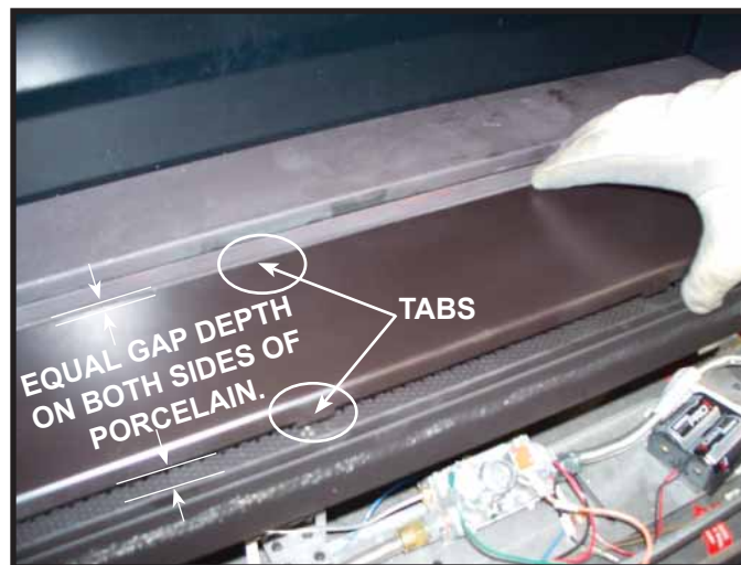
Figure 11. Placing Porcelain Base Pieces.
