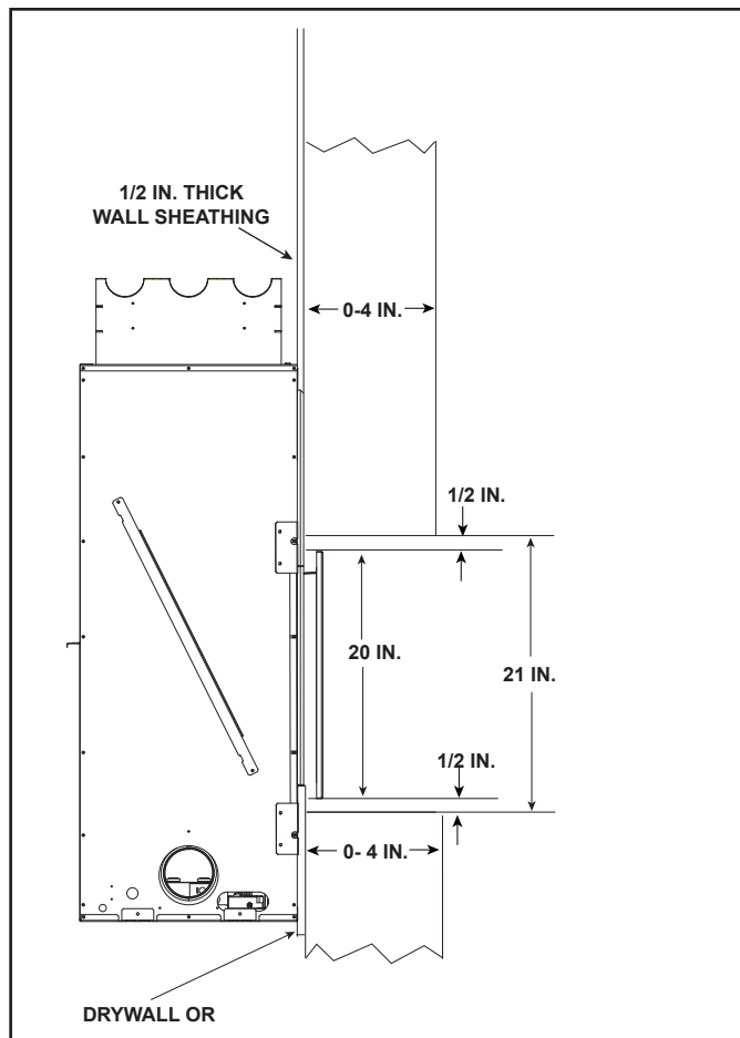
Figure 10.5 Inside Fit Method
