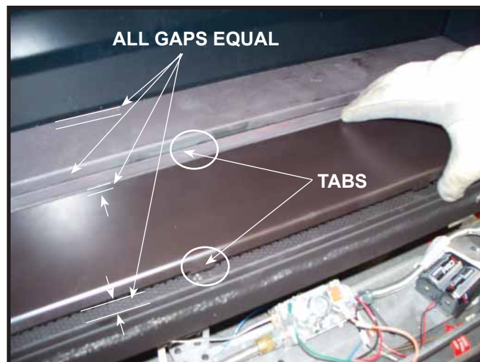
Figure 5. Placing Base Pieces.
