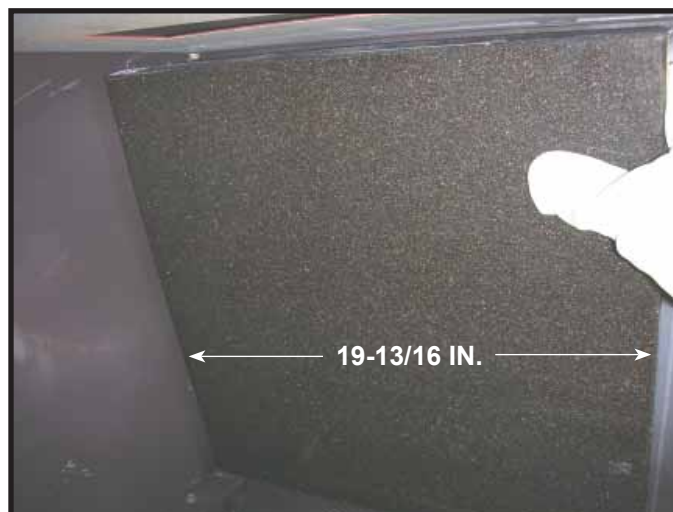
Figure 6. Placing Back Panel Piece.
