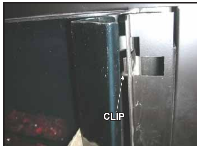
Figure 10. Installing Outside Corner Trim Piece onto Clip.
