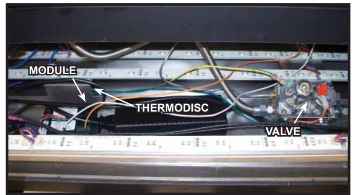
Figure 8.4 Valve Cavity
