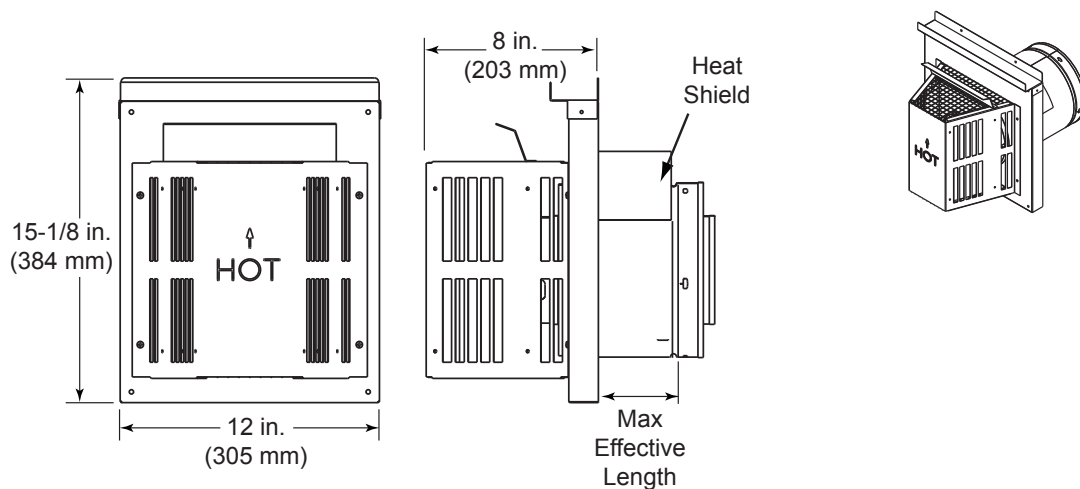
DVP-TRAP Horizontal Termination Cap
