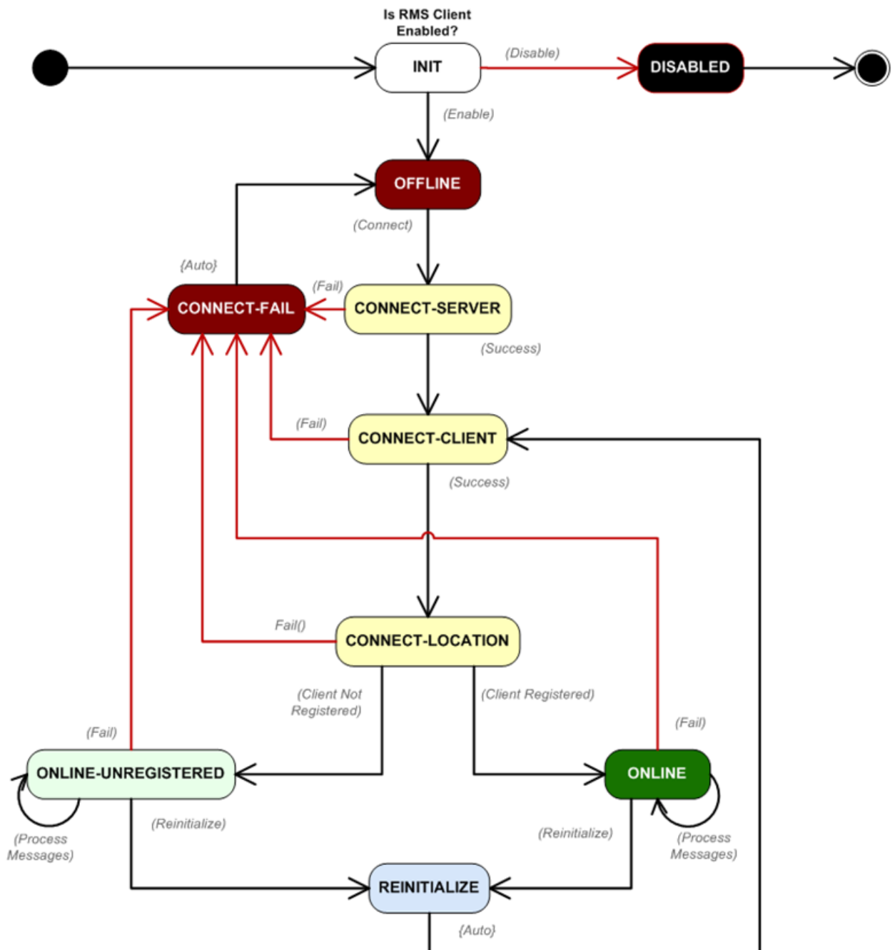
FIG. 15 Client Connection State Machine
