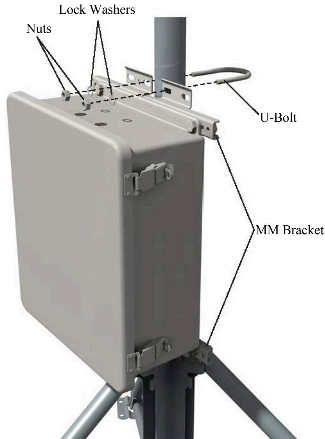
FIGURE 6-11. Enclosure with the -MM bracket
