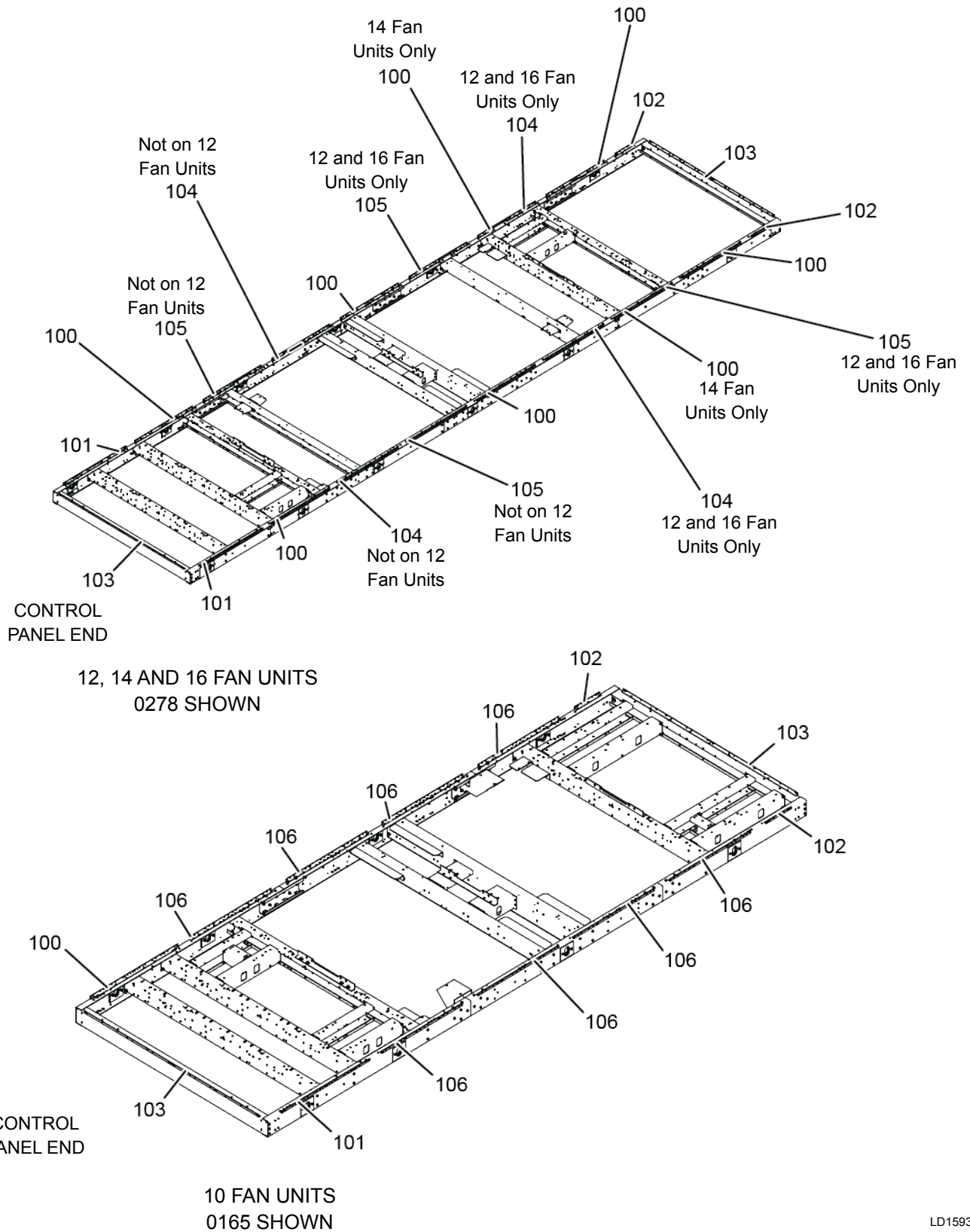
FIGURE 30 - WIRE ENCLOSURE KIT COMPONENTS - BOTTOM (GRILLE MOUNTING ANGLES), MODELS 0165 THRU 0198, 0213 THRU 0303, AND 0323 (10, 12, 14 AND 16 FANS)
