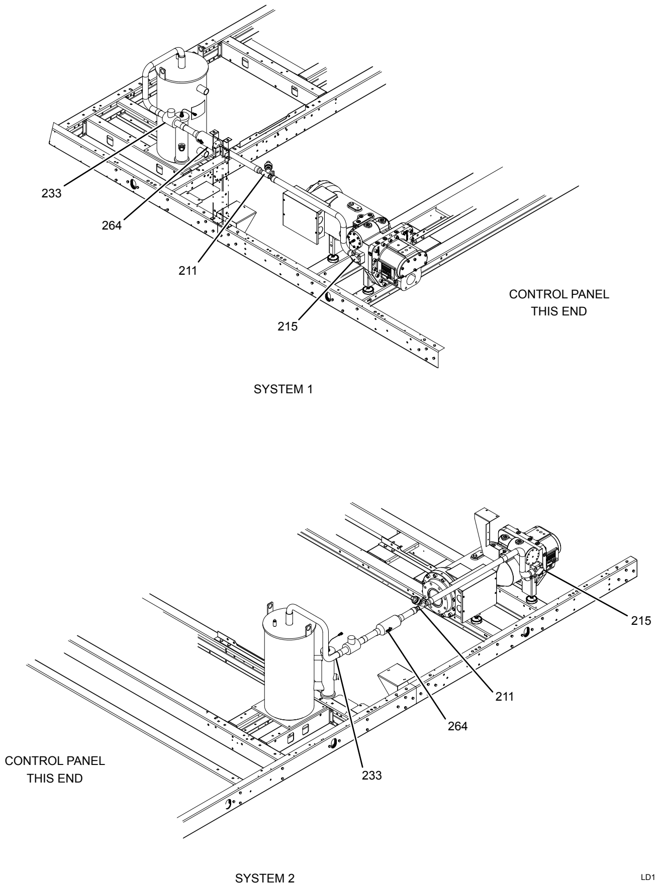
FIGURE 6 - REFRIGERATION CIRCUITS
