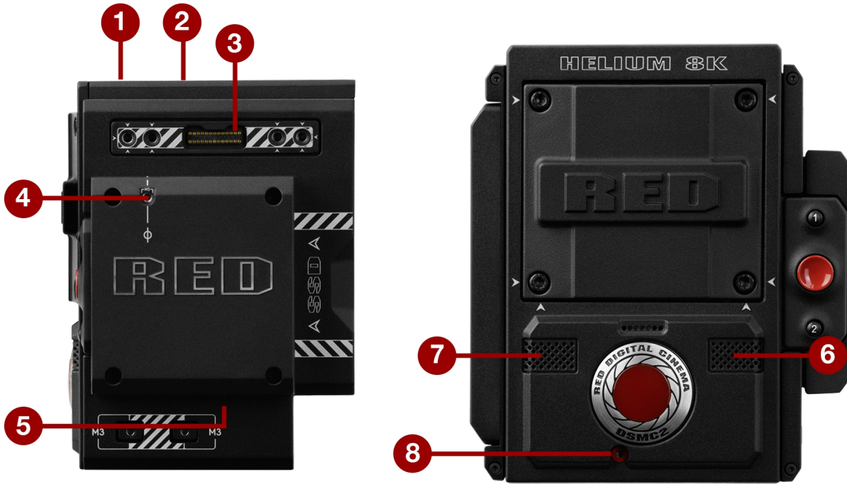
Figure: BRAIN Ports and Features
