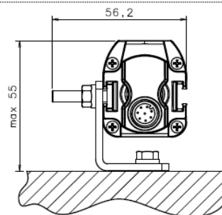
MOUNTING B
