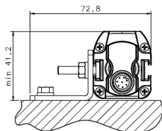
MOUNTING A
