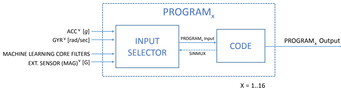
Figure 5. Program block
