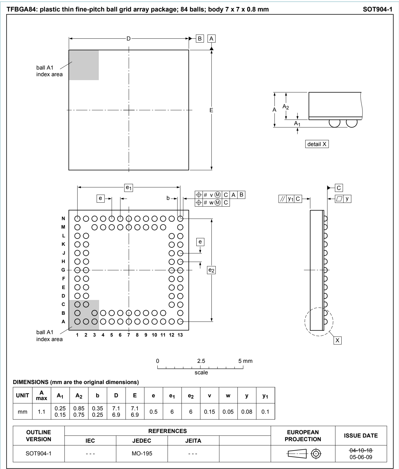
Fig. 1. Package outline TFBGA84 (SOT904-1)
