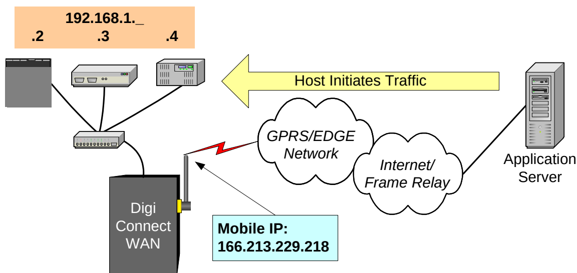
Figure 2 - TCP Port Forwarding
