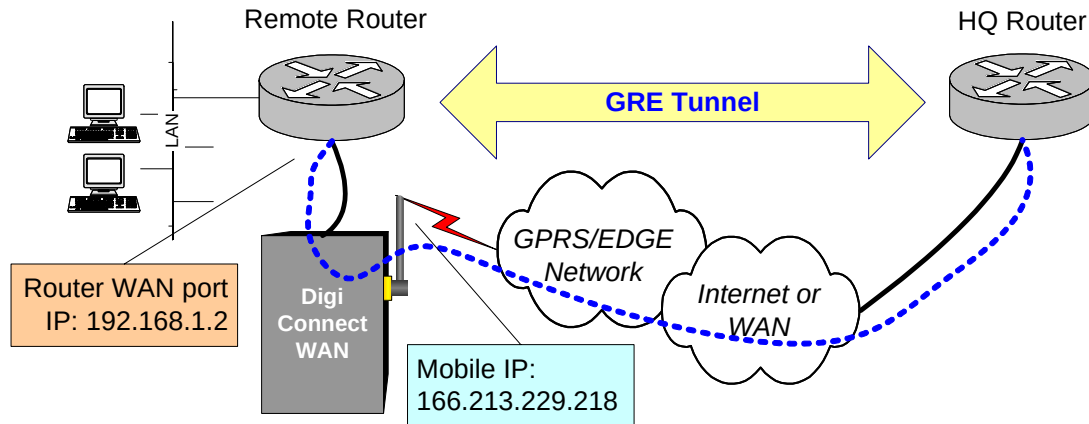
Figure 1 - GRE Forwarding
