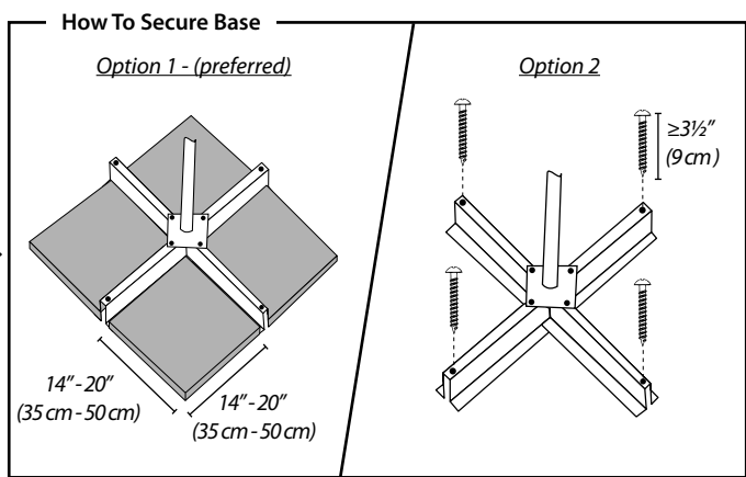
Option 1 - Position (4) - 14"-20" (35 cm - 50 cm) paver stones onto the base before raising canopy. Option 2 - Base can be secured to decking/patio with bolts or deck screws at least 3 1/2" (9 cm) long.
