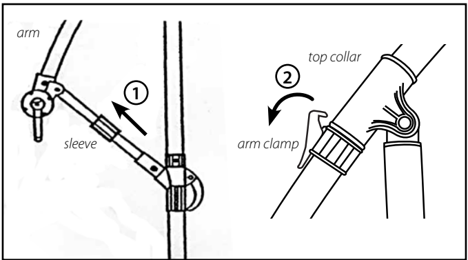
A. 1: With the canopy open, slide sleeve up. 2: Release clamp from top collar.
