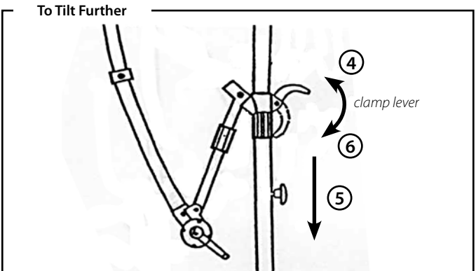
C. 4: Unlock clamp lever (up). 5: Slowly slide down to desired position. 6: Lock in place with clamp lever (down).
