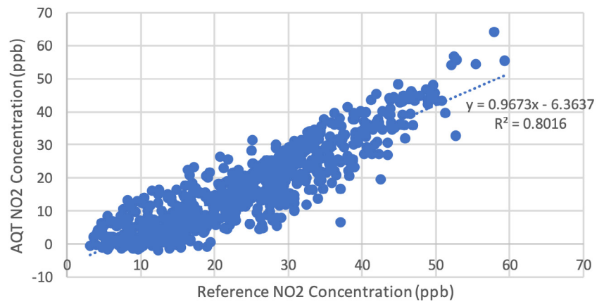
Figure B: Scatter graph illustrating the correlation between sensor and reference readings
