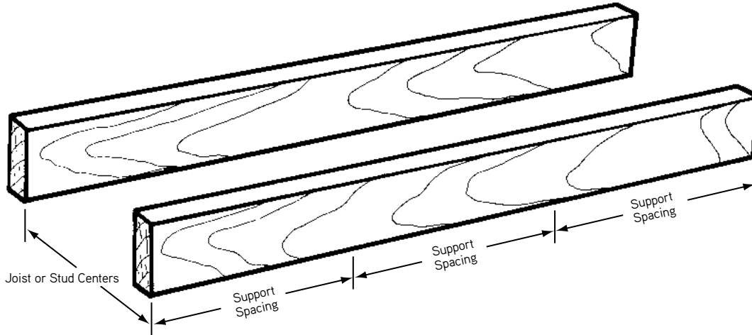
Safe Spacing of Supports for Joists or Studs Continuous Over Four or More Supports Based on use of No. 2 Grade Southern Pine or Douglas Fir-Larch
