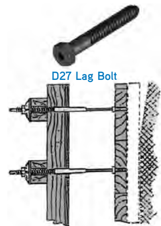
Typical Application
