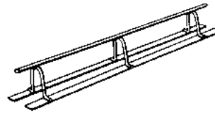
CHCP-Cont. High with Plate Manufactured to Order
