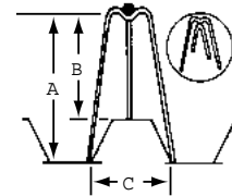
CHC Continuous High Chairs for Metal Decking Available in heights of 2" to 9" with leg spacing of 4-1/2" to 10"
